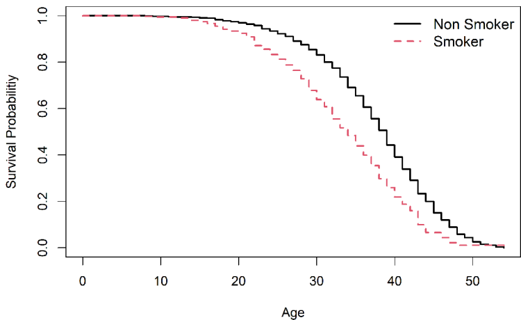
Figure 2 Kaplan-Meier Estimator of Survival Probabilities for Smokers vs. Non-Smokers
