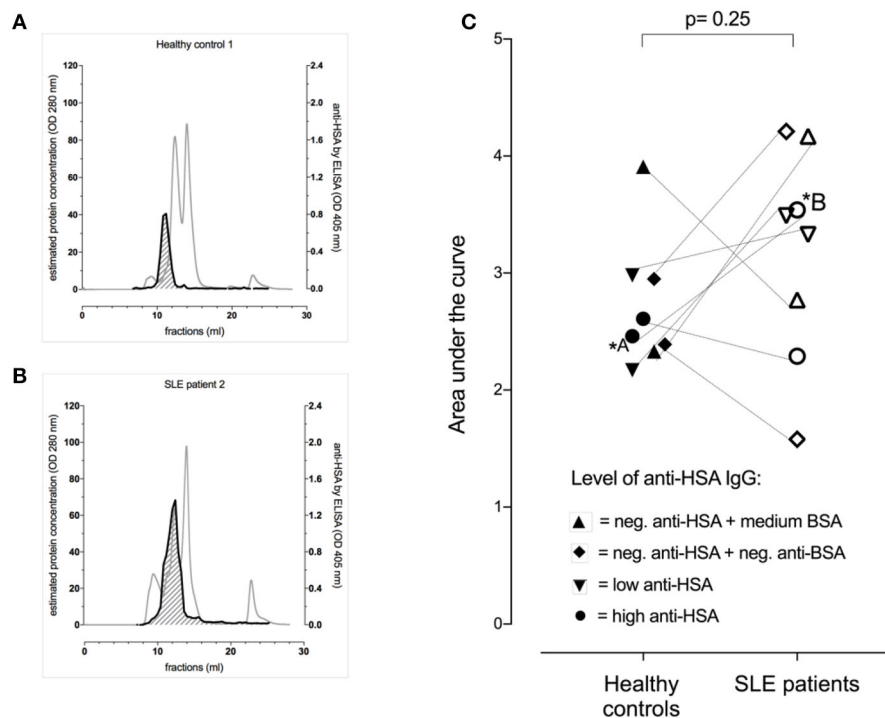
FIGURE 2 | Occurrence of albumin-IgG complexes in representative serum profiles (gray lines) after separation by FPLC of one of the healthy controls ( A ) and the corresponding (matched for anti-BSA IgG and anti-HSA IgG levels) SLE patient ( B ). Both had high levels of anti-BSA IgG and anti-HSA IgG. The dark line indicated the signal intensity for albumin (HSA)-IgG complexes with the area under the curve (AUC) being shaded (AUC of the healthy control = 2.60 vs. AUC of the matched SLE patient = 4.21). ( C ) Demonstrates pooled data of 8 SLE patients and 8 healthy controls being matched for anti-HSA and anti-BSA levels as highlighted by the use of different symbols. Overall, there was no significant difference between the SLE patients and their corresponding healthy controls, but the SLE patients tended to have more albumin (HSA)-IgG immune complexes.
