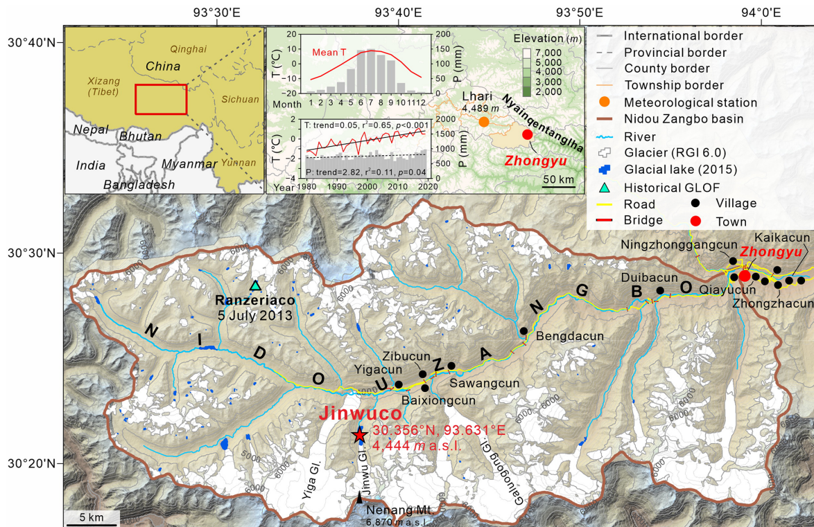
Figure 1. Location of Jinwucuo and surrounding geographic features, including terrain, rivers, glaciers, glacial lakes, settlements, and major infrastructures (roads and bridges) downstream. The climate statistics in the upper middle panel are based on the Lhari weather station, approx. 50 km away from Jinwucuo, 1980–2019. The topographic base map is based on the DEM generated from Ziyuan-3 stereoscopic pairs. The borders and location of the villages are from © Baidu Maps.
