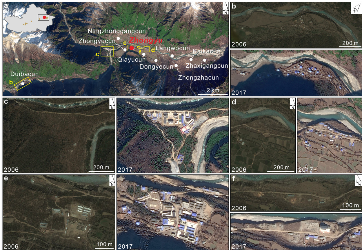
Figure 13. Examples of rapid development and expansion of the villages of lower Zhongyu township during 2006–2017. The background of panel (a) and the satellite scenes for the 2017 panels are a true-color composite Gaofen-2 image acquired on 7 December 2017. The satellite images for the 2006 panels are from © Google Earth, acquired on 30 April 2006.
