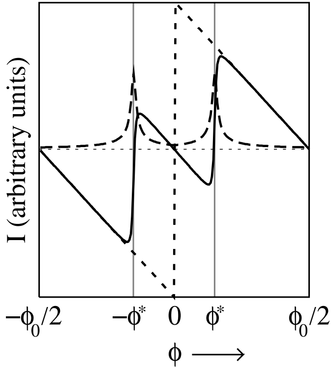
Figure 3. The persistent current (solid line) and its fluctuations (\Delta I^2)^{1/2} (dashed line) in the two-level approximation with N_r^+ even and |t| \approx 0.32w . For comparison the persistent current for N_r^+ electrons in the ring and in the absence of hybridization is shown (short dashed line). The persistent current vanishes near the hybridization points \pm\phi^* ( = \pm\phi_0/6 in the example) whereas the fluctuations have maxima near the same points, which are of the same order of magnitude as the persistent current in the absence of hybridization.
