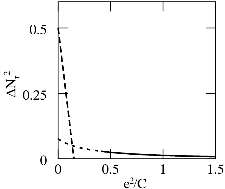
Figure 6. Particle number fluctuations as a function of e^2/C . The result in the incoherent Coulomb blockade model \overline{(\Delta N_r^2)}_{inc} (dashed line) and the off-resonant result \overline{\Delta N_r^2} for e^2/C > 2w + \Delta (solid line), continued beyond its range of validity (short dashed line) are shown for \phi = \pm\phi_0/4 , |t| = 0.02 , w = 0.1 , \Delta = 0.2 . All energies are given in units of the band width \Lambda .
