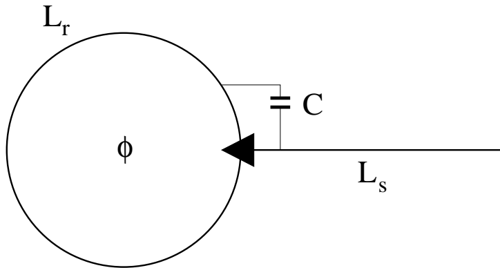
Figure 1. A ring pierced by a flux \phi and coupled to a (finite length) side stub. The triangle represents the a three way tunneling junction and the Coulomb interaction is taken into account via the capacity C .
