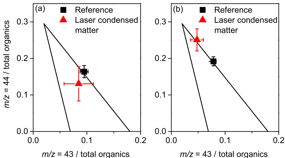
FIG. 5. Fraction of highly ( m/z = 44 , mainly \text{CO}_2^+ ) and less oxygenated ( m/z = 43 , mainly \text{C}_2\text{H}_3\text{O}^+ ) organics among the total organics, in particles detected during the reference period (black) and the laser-condensed particles, that is the difference of measurement with and without the laser (red), for (a) the main experiment and (b) when spraying water in a low RH atmosphere (b). The two black lines encompass the region where most atmospheric data are found to date[32].
