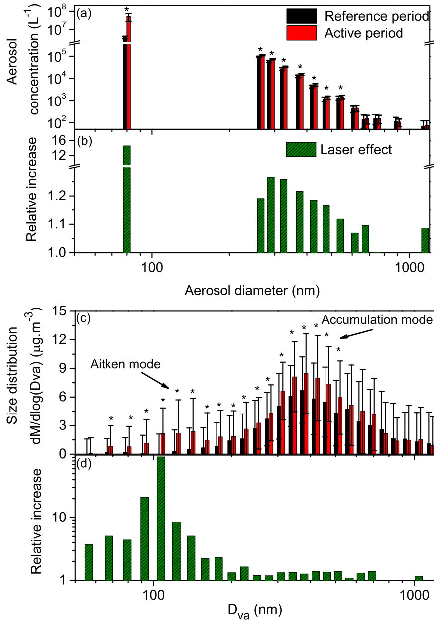
FIG. 3. Evolution of the aerosol size distribution under laser illumination. (a) Aerosol size distribution between 250 and 900 nm during both reference and active periods measured by the Grimm optical particle sizer, and concentration of 25 - 300 nm particles measured by the Nanocheck (column centered at the mean diameter 80 nm); (b) Corresponding relative increase induced by the laser; (c) Dry particle size distribution (total mass detected by the AMS, calculated as the sum of nitrate, sulfate, organics, ammonium and chloride) during both reference and active periods and (d) Corresponding relative increase induced by the laser. D_{va} is the vacuum aerodynamic diameter. Stars denote size classes where the effect of the laser is statistically significant ( \alpha \leq 0.01 , see text for details). Error bars correspond to one standard deviation.
