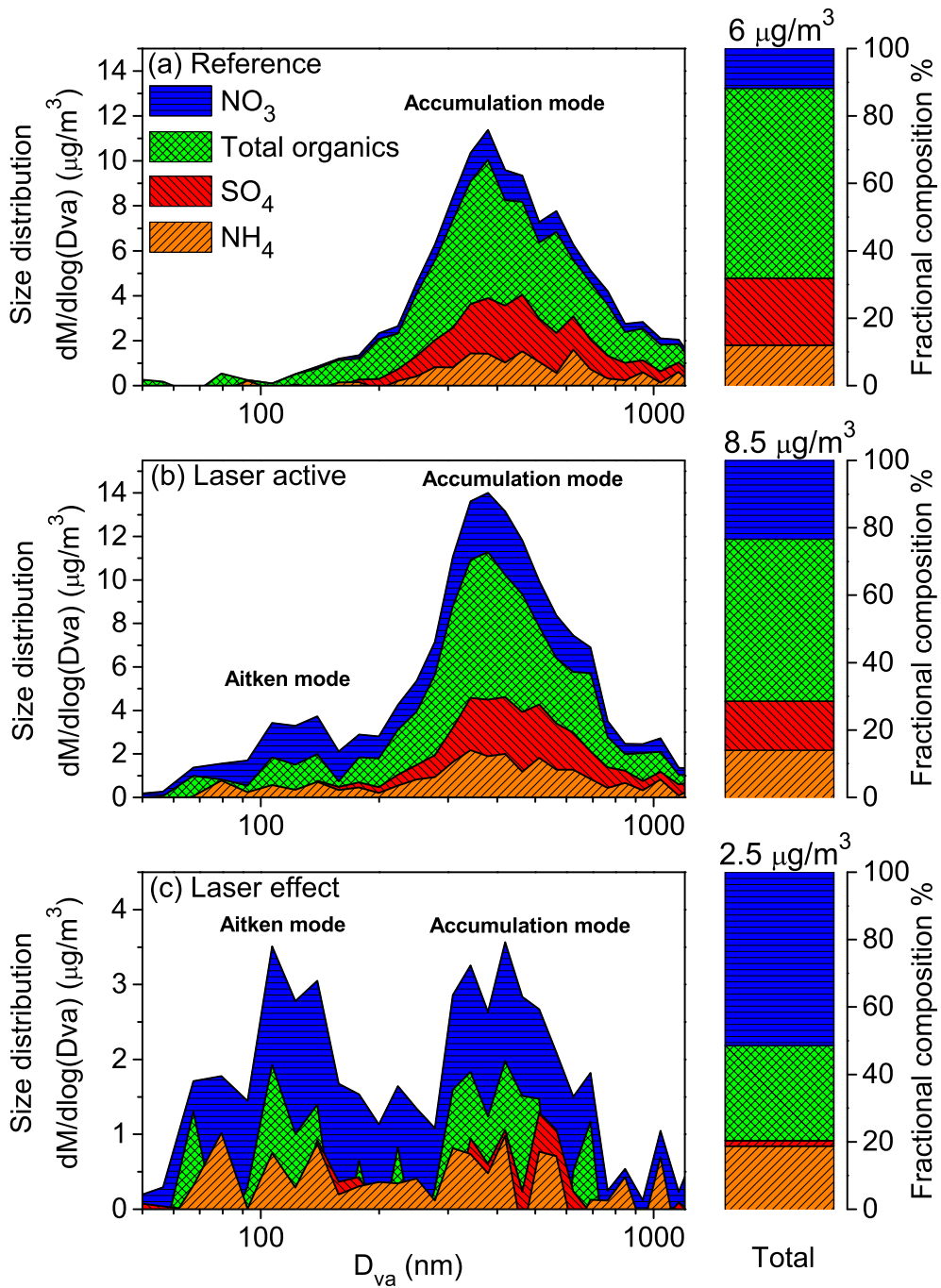
FIG. 4. Mass distribution of the measured condensable species within the size distribution during (a) the reference period and (b) the laser active period. (c) Difference between the active and reference periods, displaying the condensation effect of the laser. D_{va} is the vacuum aerodynamic diameter.
