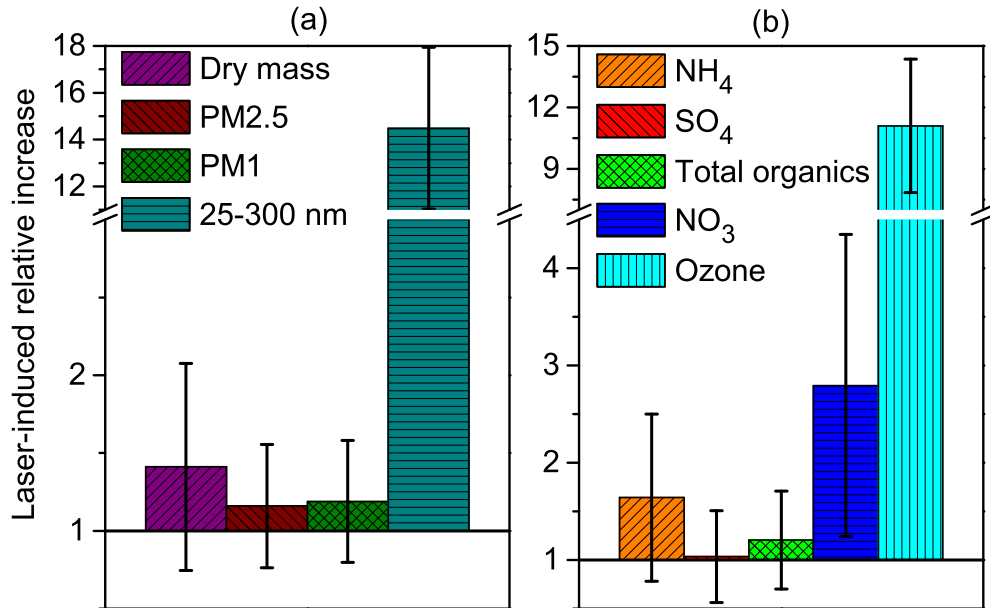
FIG. 2. Laser-induced relative increase of (a) the aerosol dry mass concentration measured by the AMS (sum of sulfate, nitrate, organics, ammonium and chloride for vacuum aerodynamic diameters between 60 and 600 nm), the PM1 and PM2 mass concentration measured by the optical sizer and the number concentration of 25 to 300 nm particles detected by the nanoparticle sensor, and (b) the mass concentration of several condensable components detected by the AMS, as well as atmospheric ozone concentration. Error bars correspond to the sum of the relative standard deviations of the values measured with and without laser.
