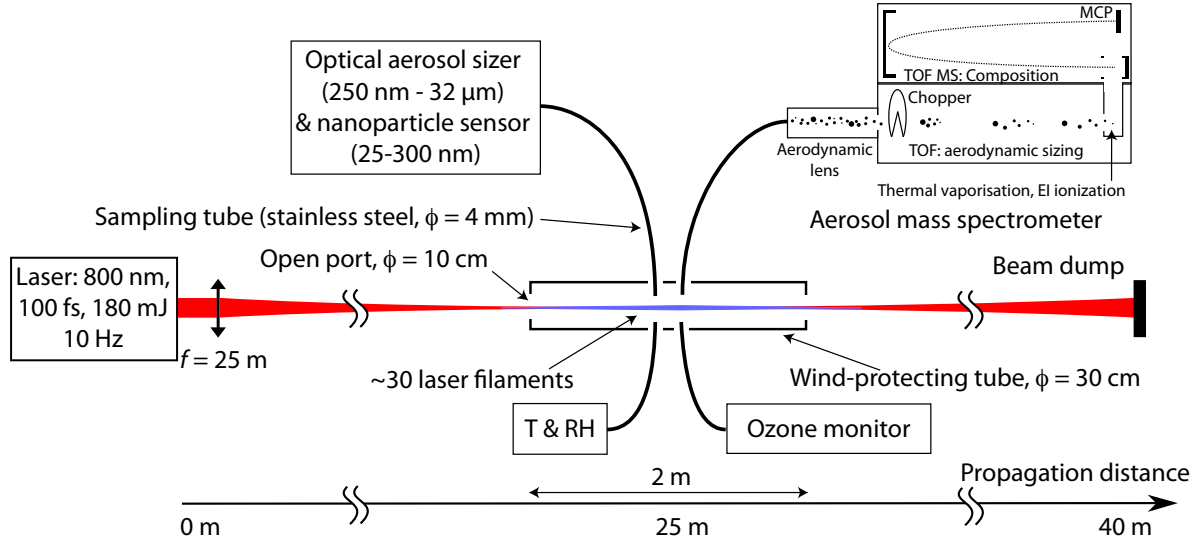
FIG. 1. Experimental setup. TOF: Time of flight; MS: Mass spectrometer; EI: Electron impact; MCP: Micro-channel plate.
