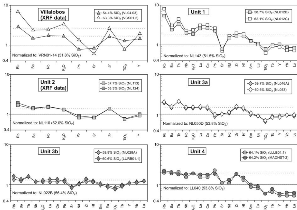
Figure 19. Multi-element spidergrams illustrating the compositions of the two most evolved samples of each unit, normalized to a mafic sample of the same unit. Dotted lines represent the estimated maximum level of enrichment due to closed-system differentiation.
