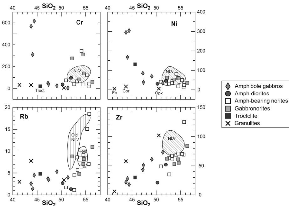
Figure 15. Selected trace element composition of NLV xenoliths and fields of NLV mafic magmas (MgO>5 wt%) shown for comparison (fields of Holocene and older units are distinguished for Rb). Note elevated Cr and Ni contents of amphibole gabbros and basalt-like composition of norites and gabbronorites. Labels for granulites: Fe=iron-oxide-rich granulite; Cor=cordierite-corundum granulite; Opx=orthopyroxene-rich granulite. All elements as determined by XRF (see Table 1).
