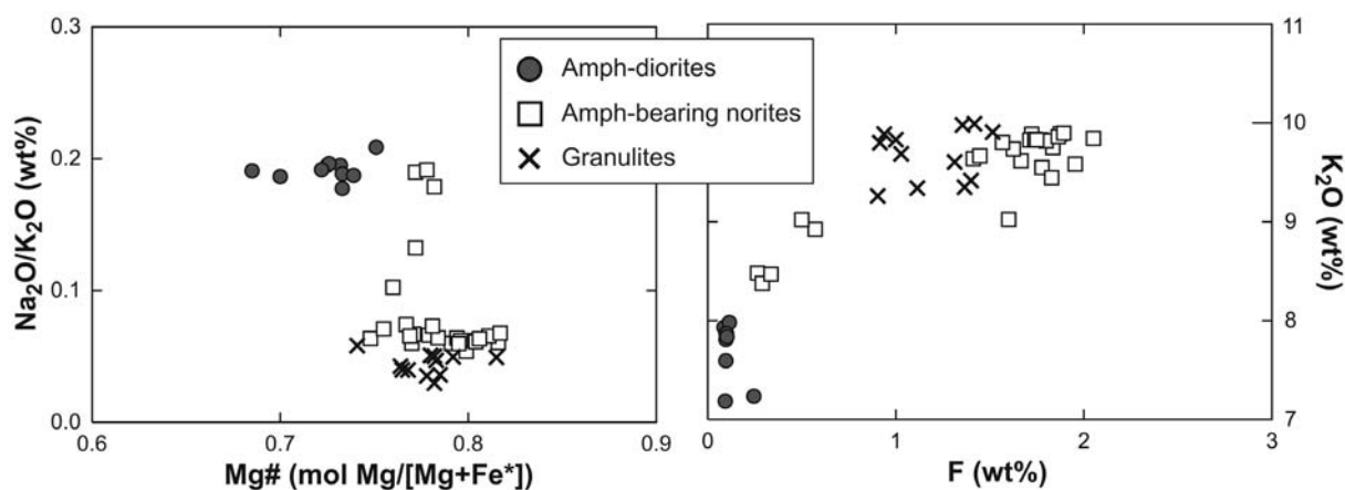
Figure 13. Biotite (phlogopite) compositions. Note the high F and K 2 O contents of biotite crystals in norites and granulites (relative to those of diorites), which suggests crystallization from a highly evolved residual liquid or partial melt. Fe* = total Fe.
