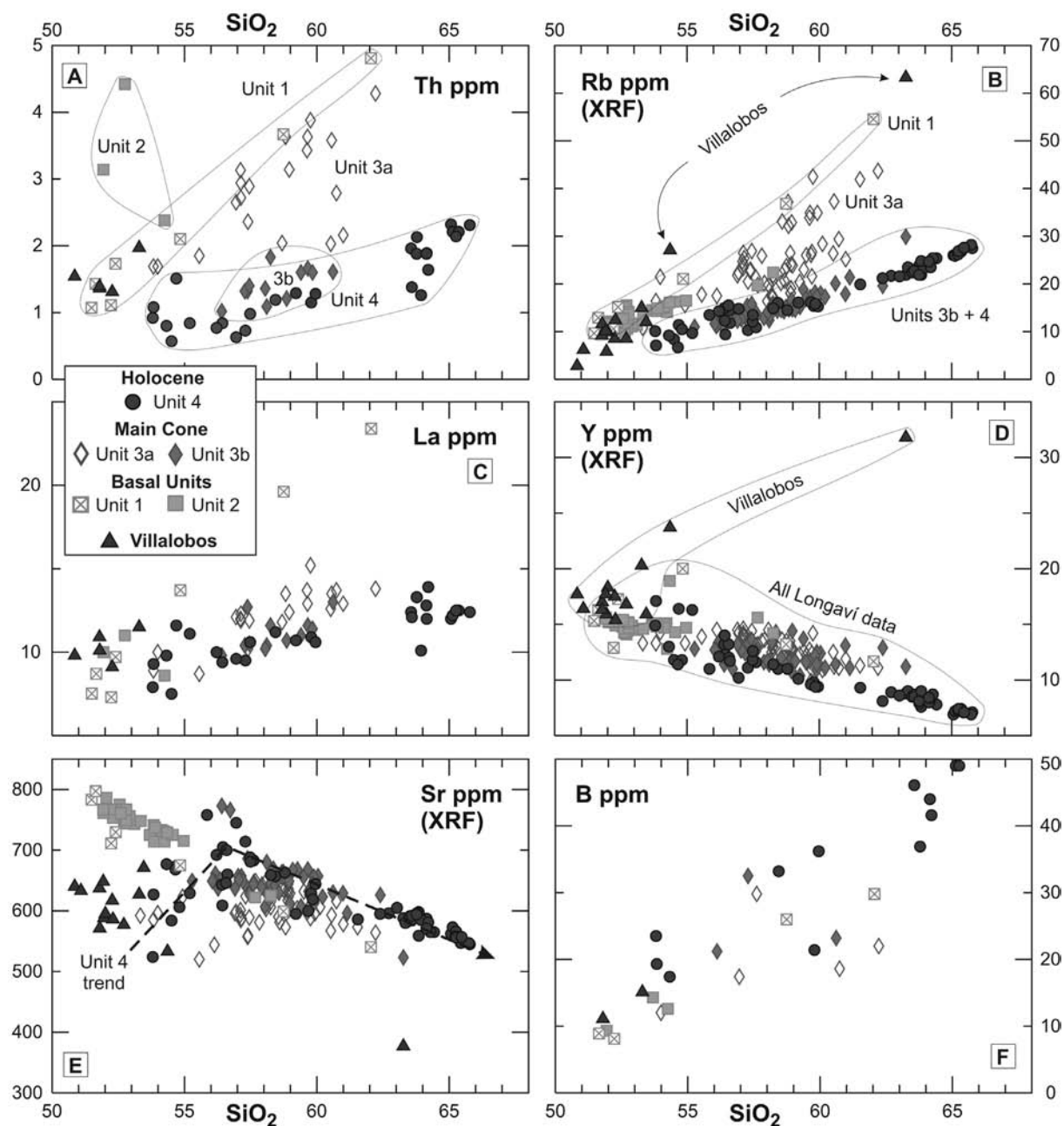
Figure 7. Selected trace elements for Longaví and Villalobos lavas. A sustained decrease in incompatible element content (for a given SiO 2 content) from old to young units is clearly seen for Th, Rb and La, similarly to K 2 O, although unit 2 lavas contain high Th contents (as well as U and Pb). Boron shows an opposite tendency of higher contents in young units. Y decreases with increasing SiO 2 for in all Longaví units, but increases in Villalobos lavas. Note the inflection in Sr trend for Unit 4 at 57% SiO 2 , analogous to Al 2 O 3 abundances. Th and La as determined by ICP-MS, B by ICP-AES; Y and Rb by XRF as specified.
