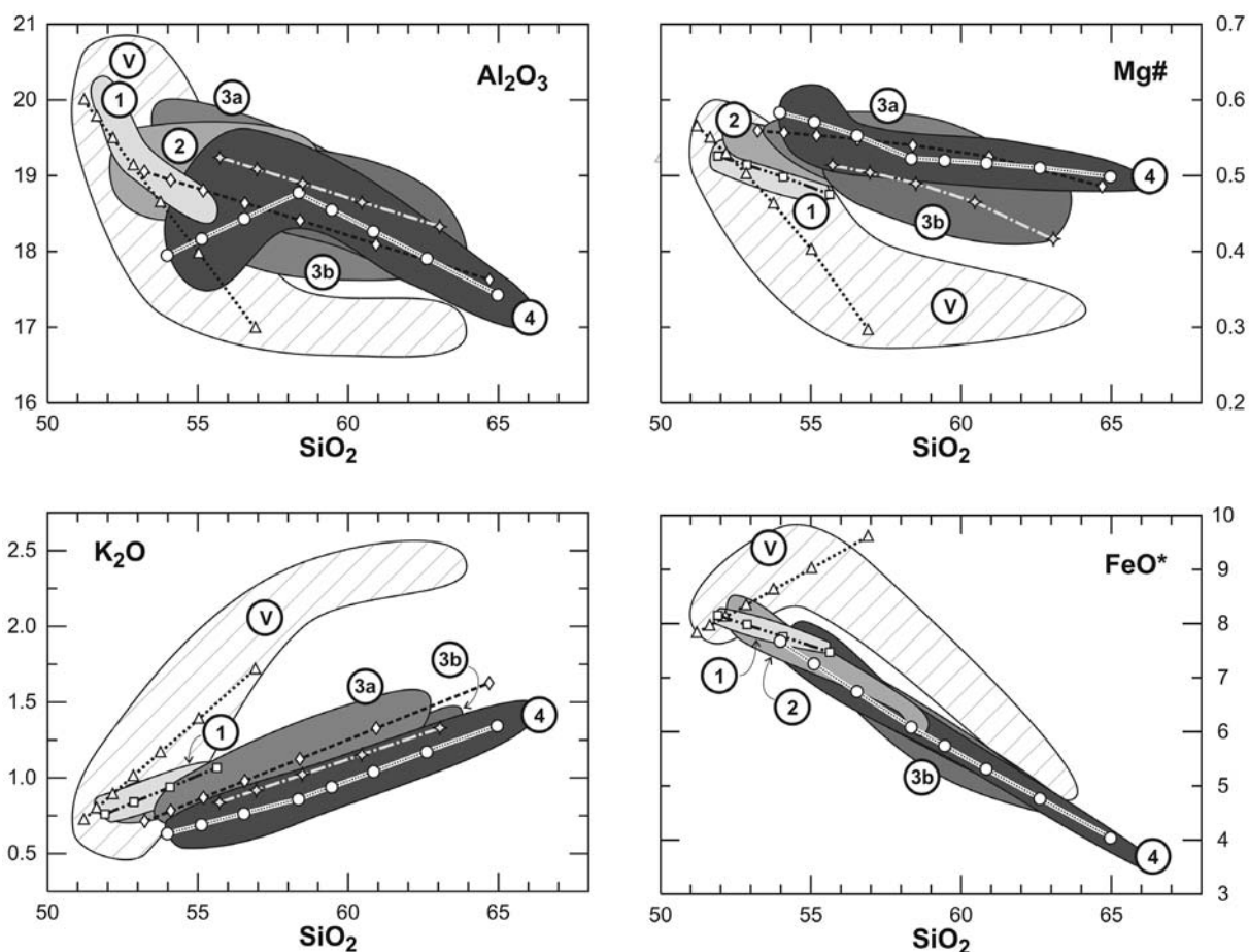
Figure 16. Mass-balance fractionation models for Villalobos and NLV units. Data normalized to 100%, all iron as FeO. Model parameters in Table 2 and Figure 6.
