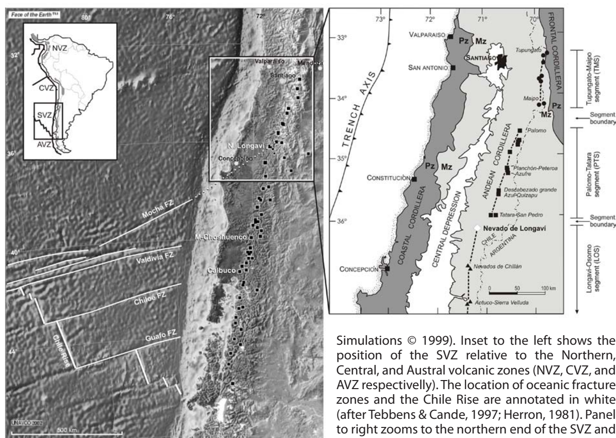
Figure 1: Location of Nevado de Longaví volcano and some other volcanic centers of the SVZ. Digital elevation model is reproduced from http://jules.unavco.ucar.edu (Face of the Earth is a registered trademark, ARC Science
