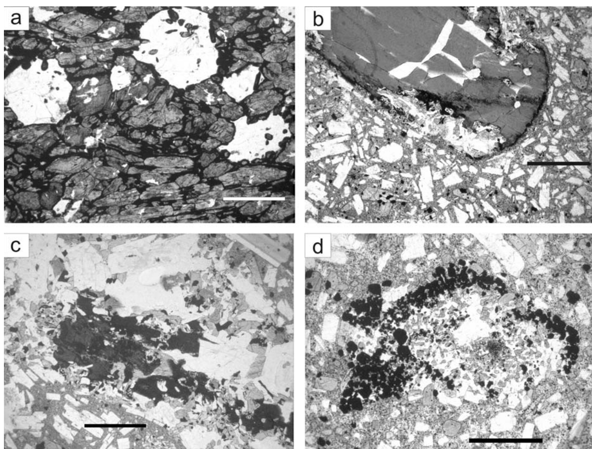
Figure 6: a) Cumulate texture in a gabbroic enclave (NL 120E). Note alignment of dark amphibole crystals and small amphibole inclusions within plagioclase (clear). Amphibole phenocrysts in Longaví magmas are replaced to varying extents by reaction products. b) Fine-grained dusty magnetite amphibole breakdown zone localized along the grain margin. c) More advanced reaction involving extensive replacement of the grain interior. d) Complete replacement of an amphibole grain wherein the original outline of the amphibole is marked by concentrations of oxides. Scale bars = 1 mm.
