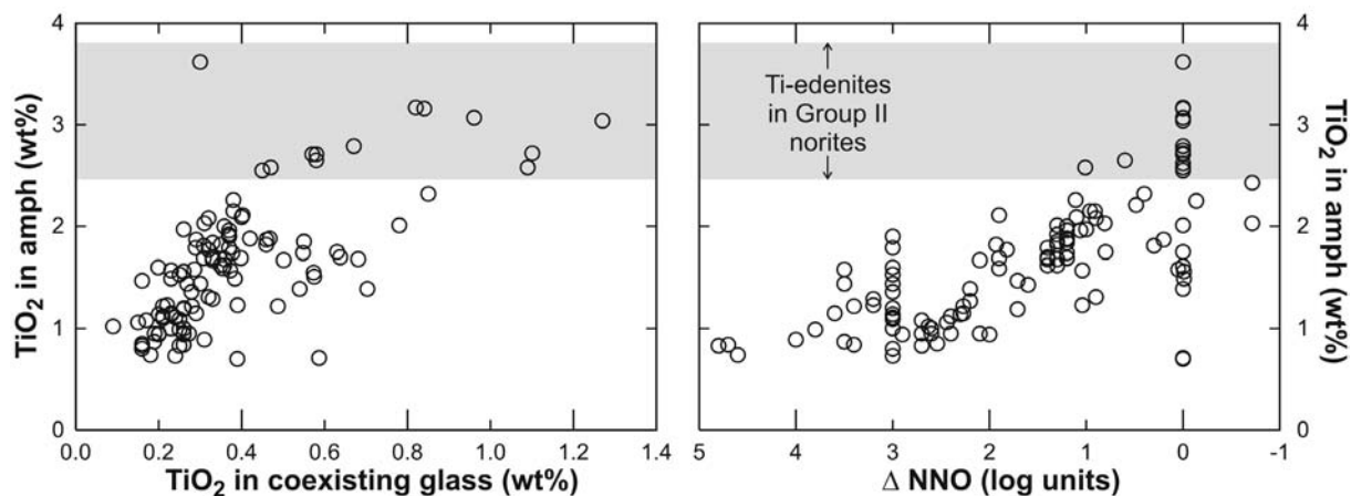
Figure 22. TiO 2 content of experimental amphiboles as a function of TiO 2 in the coexisting glass and of Δ-NNO conditions of the experiments. Range of TiO 2 content of amphiboles in Group II norites shown in gray bands. Data sources as in Figure 20.
