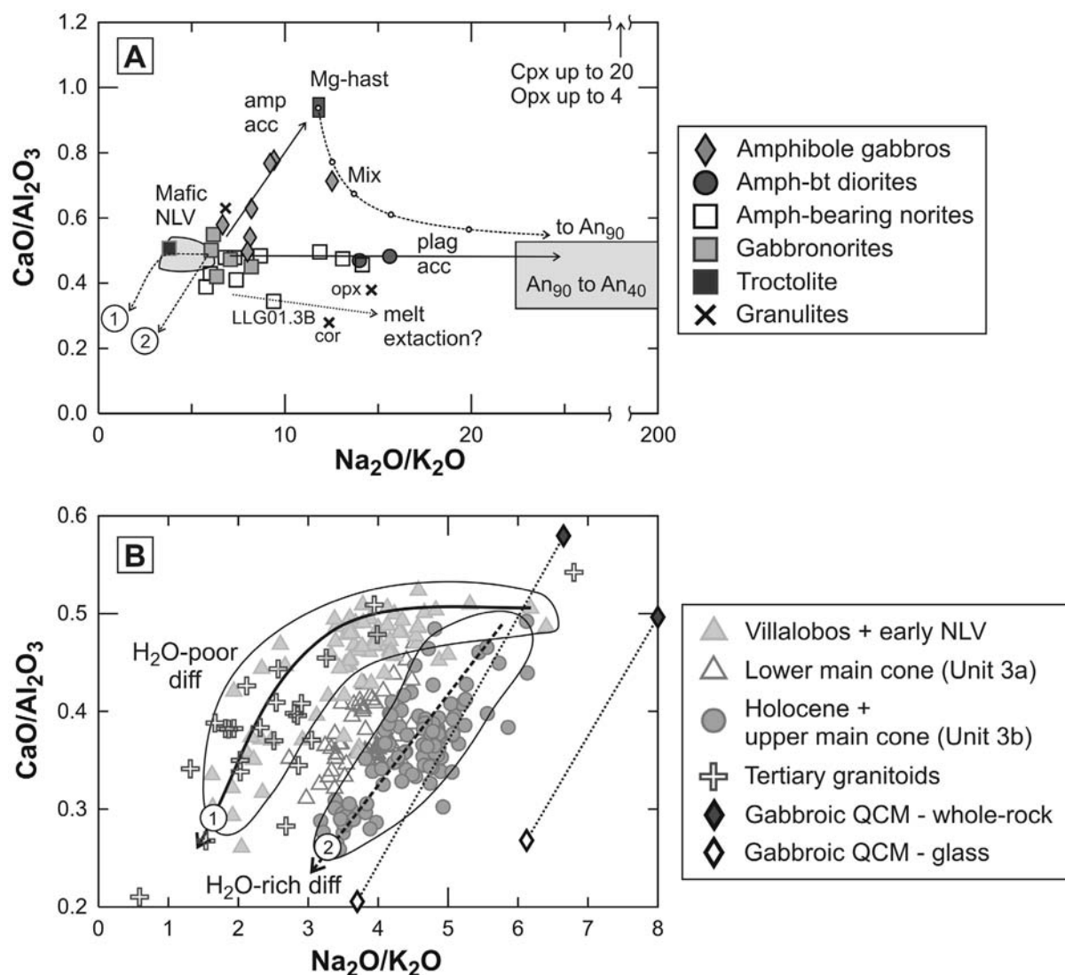
Figure 23. Summary diagram with the proposed processes recorded in NLV xenoliths. A: A reference starting composition close to NLV mafic lavas is presented in the shaded field. Amphibole accumulation towards average Mg-hastingsitic composition (box labeled Mg-hast) is recorded in amphibole gabbros. Sample away from the depicted trend lies in the mixing line between amphibole and \text{An}_{90} plagioclase. Increasing \text{Na}_2\text{O}/\text{K}_2\text{O} ratio at constant \text{CaO}/\text{Al}_2\text{O}_3 for amph-diorites and norites is consistent with plagioclase accumulation (box includes \text{An}_{40} to \text{An}_{90} plagioclase compositions). Increasing \text{Na}_2\text{O}/\text{K}_2\text{O} accompanied by decreasing \text{CaO}/\text{Al}_2\text{O}_3 could indicate melt extraction as is suggested by two of the granulites and a norite sample with advanced partial melting. B: Early extraction of plagioclase from basalts produces the water-poor differentiation path (1) observed in early Longaví units and pre-Longaví lavas (and the Tertiary plutons), whereas early amphibole crystallization produces the water-rich differentiation trend (2) depicted by young NLV lavas.
