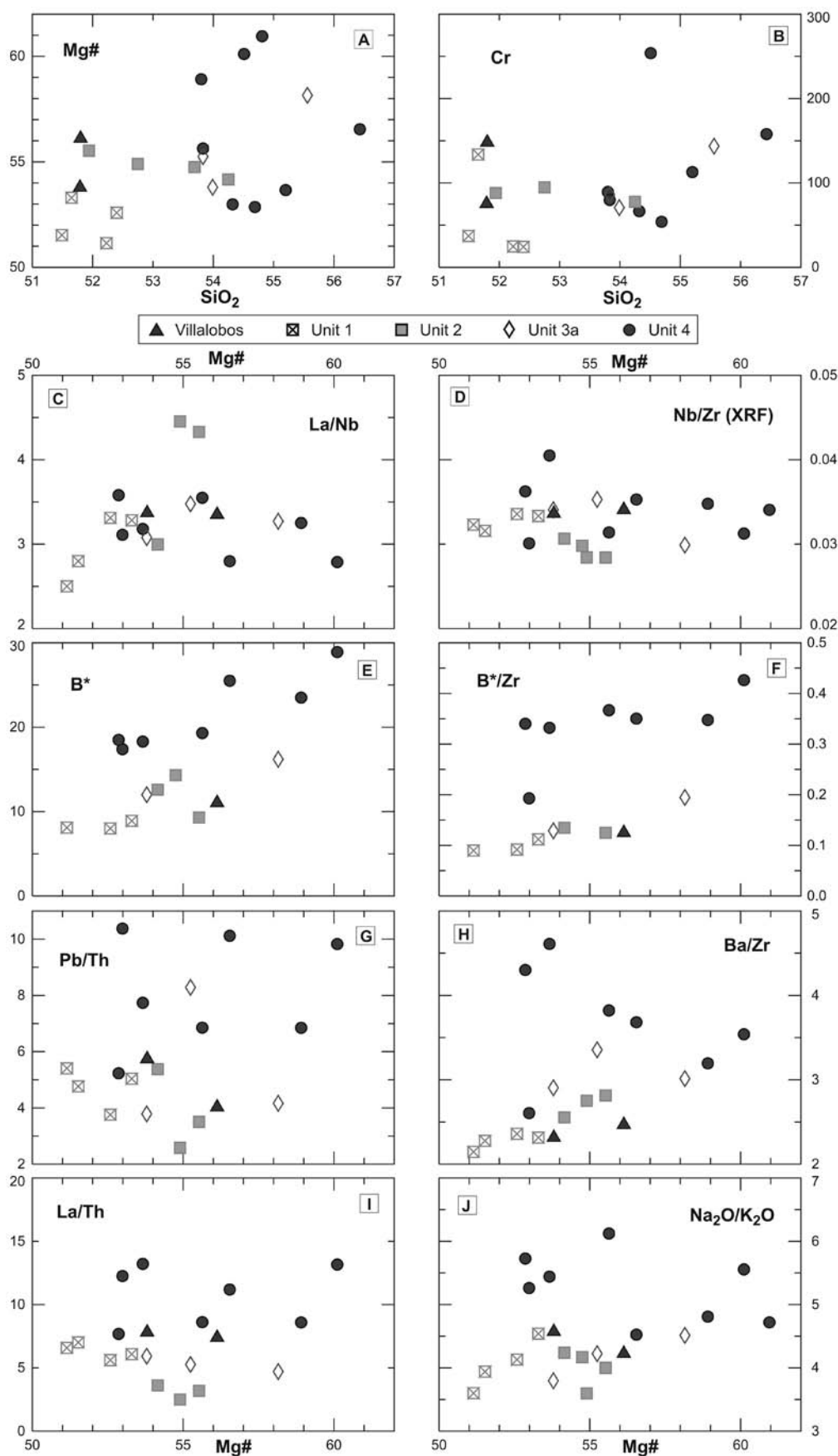
Figure 21. Variation chemical diagrams for samples with MgO > 4.5 wt%. A and B: Holocene mafic enclaves have Mg# and Cr contents comparable to those of older basalts despite their higher SiO_2 contents. C and D: Ratios of similarly immobile elements (La/Nb, Nb/Zr), thus probably characteristic of the mantle source, are constant for mafic magmas from all units. E through J: Concentration of the highly fluid-mobile element B and ratios of mobile to immobile element are high in Holocene enclaves compared to older basalts. B* is combined ICP-AES and ICP-MS data (see table 1).
