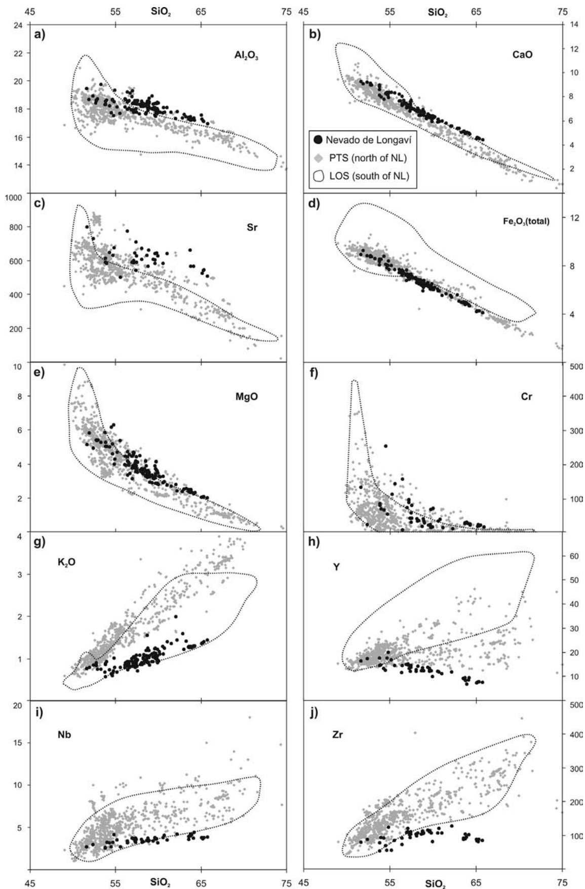
Figure 7: Major and trace element variations as a function of wt% SiO 2 . The data base used as reference includes 383 analyses from the LOS and 910 from the PTS (Fig. 3), 638 of which are from the Tatara-San Pedro complex. Data include literature analyses (various references in text) as well as unpublished data from ongoing projects at the University of Geneva.
