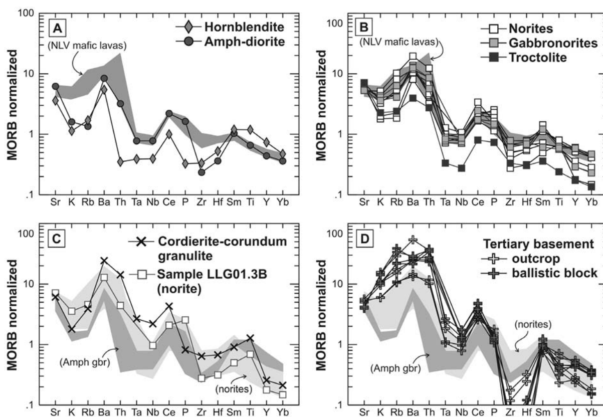
Figure 17. MORB-normalized (Pearce, 1983) spidergrams for the different types of xenoliths at NLV. A: Plagioclase-bearing hornblendite and amph-diorite compared to the range of NLV mafic magmas ( \text{MgO} > 5 wt%). B: Group II xenoliths (except granulites). Note the overlap of most samples with the composition of NLV lavas. C: Cordierite-corundum granulite compared to Group I and II NLV xenoliths (shaded fields); also shown composition of a norite with advanced partial melting that shows similar K, Rb, Y and Yb depletions. D: Range of compositions from tertiary plutonic basement.
