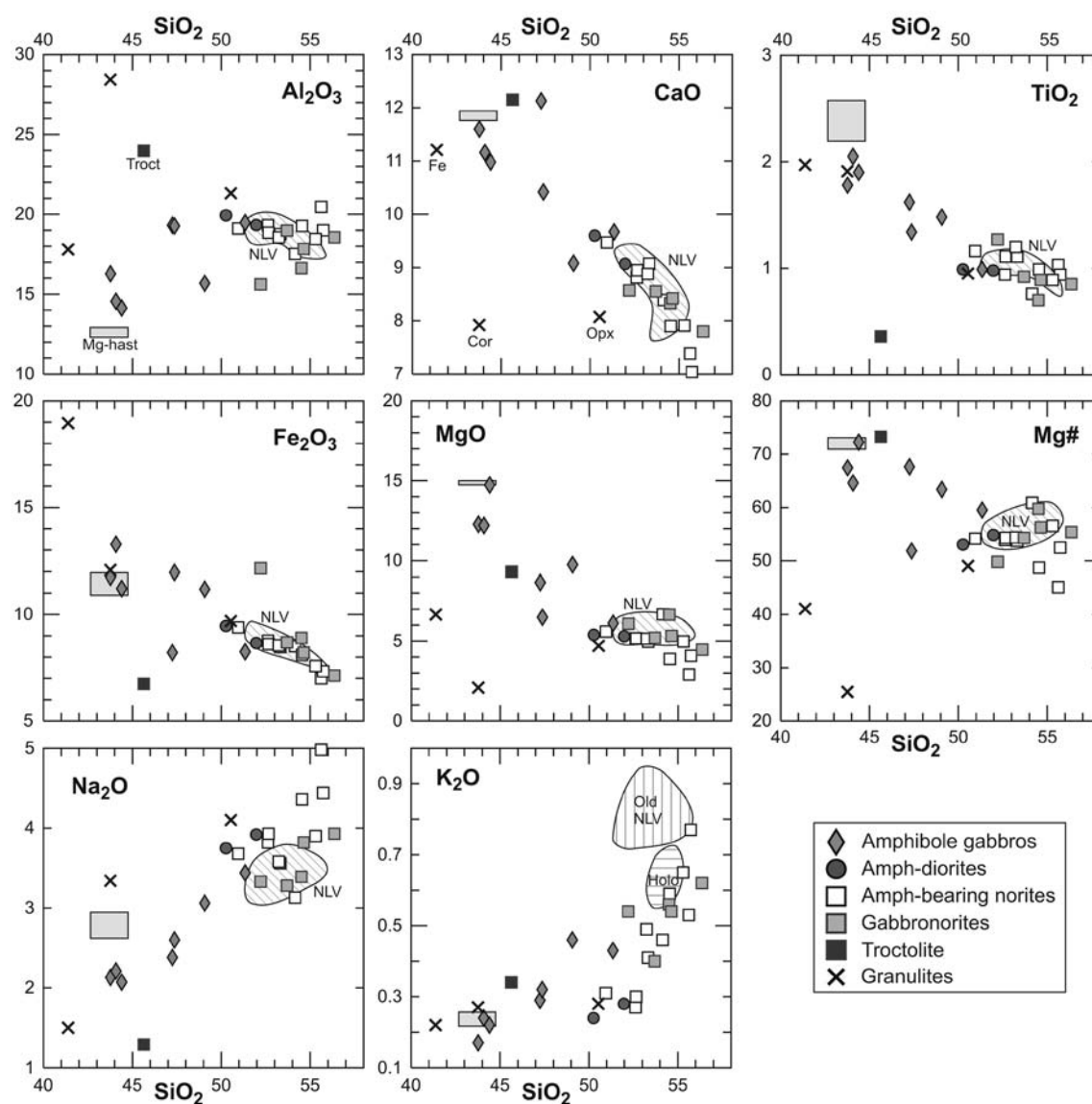
Figure 14. Major element composition of NLV xenoliths. The compositional fields of mafic NLV magmas (MgO > 5 wt%) are shown in fields labeled "NLV" (fields of Holocene and older units are distinguished for K 2 O). Note that amphibole gabbros extend from basaltic compositions to the average compositions of Mg-hastingsite amphiboles (gray rectangles), whereas most Group II xenoliths have compositions similar to NLV mafic magmas. Troctolite composition is consistent with olivine and plagioclase accumulation. Granulites are more diverse, with non-magmatic compositions. Labels for granulites: Fe=iron-oxide-rich granulite; Cor=cordierite-corundum granulite; Opx=orthopyroxene-rich granulite.
