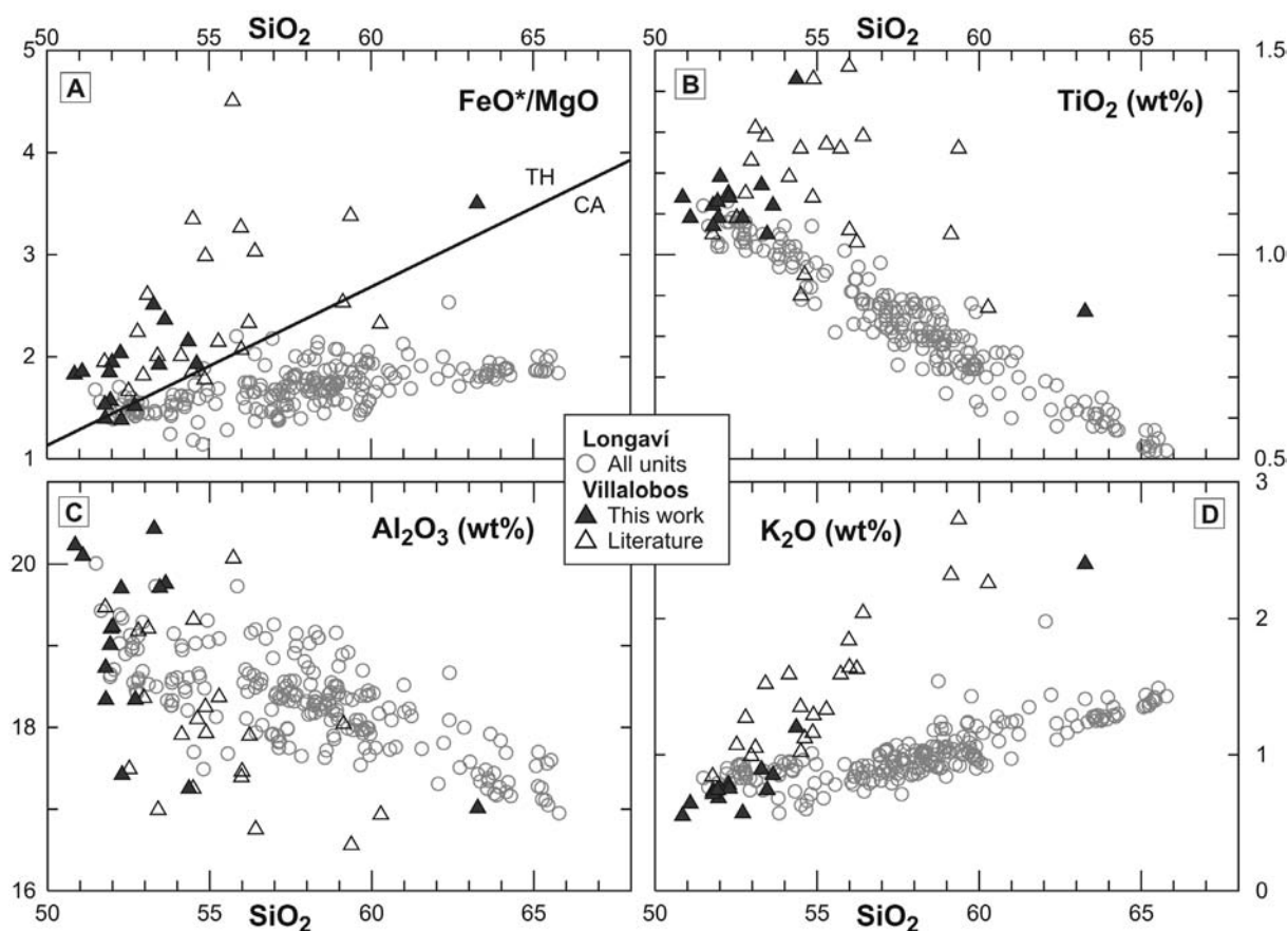
Figure 4. Major element variations of pre-Longaví volcanics (Villalobos volcano) compared to NLV magmas. Note early FeO* and TiO 2 enrichment of Villalobos lavas, typical of tholeiitic liquid lines of descent (dividing line in A is from Miyashiro, 1974). Compared to Longaví, Al 2 O 3 in Villalobos lavas (as well as MgO and CaO) decreases more abruptly and K 2 O (and Na 2 O) increase more steeply with increasing differentiation. Literature analyses are from Gardeweg (1980) and Muñoz and Niemeyer (1984).
