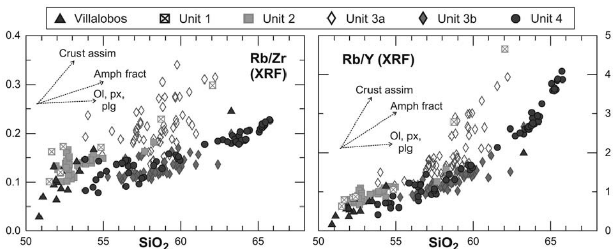
Figure 20. Rb/Zr and Rb/Y ratios of Villalobos and NLV lavas. Vectors of crustal assimilation, amphibole fractionation, and anhydrous assemblage fractionation are proposed.
