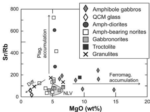
Figure 21. MgO vs. Sr/Rb plot indicating the trends of plagioclase and ferromagnesian phases accumulation. Also a trend of magmatic differentiation (Diff.) is proposed. Shaded field represents the compositions of NLV mafic magmas.
