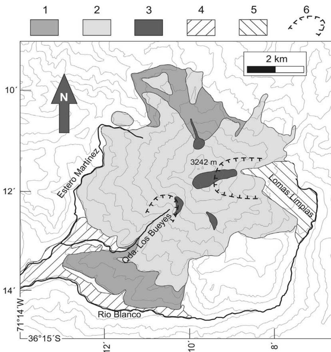
Figure 4: Schematic map of Nevado de Longaví volcano showing the units discussed in the text. 1) Early units, mainly basaltic andesitic lava flows. 2) Main cone andesites. 3) Summit area andesitic to dacitic domes, central dome of presumably Holocene age. 4) Pre-Holocene terrace deposits associated to Los Bueyes sector collapse and Martínez and Río Blanco streams. 5) Holocene pyroclastic deposits of Lomas Limpias collapse bowl. 6) Collapse scars. Contour curves every 200 m.
