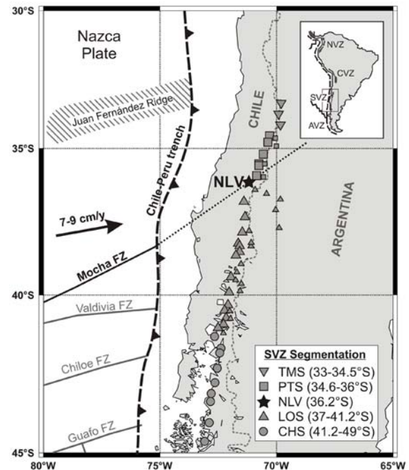
Figure 1. Location of the Nevado de Longaví volcano (star labeled NLV) in the Southern Volcanic Zone (SVZ). Location of SVZ volcanic centers shown with different symbols for different segments as defined in Chapter 2.
