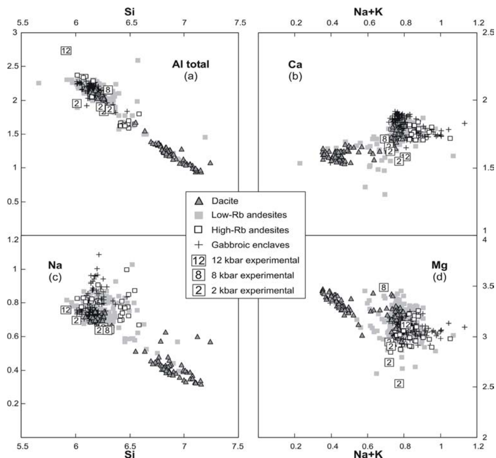
Figure 12: Chemical compositions of amphiboles in lavas, pyroclastic units and gabbroic enclaves from Nevado de Longaví. Values are in cations per formula unit calculated on a 13-cation basis. Also included for comparison are the chemical compositions of amphiboles crystallized in experiments (12 kbar experiment from Müntener et al. , 2001; 8 kbar experiment from Grove et al. , 2003; 2 kbar experiments from Grove et al. , 1997 and Grove et al. , 2003).
