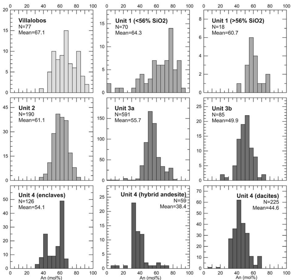
Figure 11. Histograms of plagioclase compositions (in terms of An mol%) for the units discussed in the text. Mafic and evolved samples from Unit 1 are shown separately, as well as Holocene dacites, andesite, and mafic enclaves.
