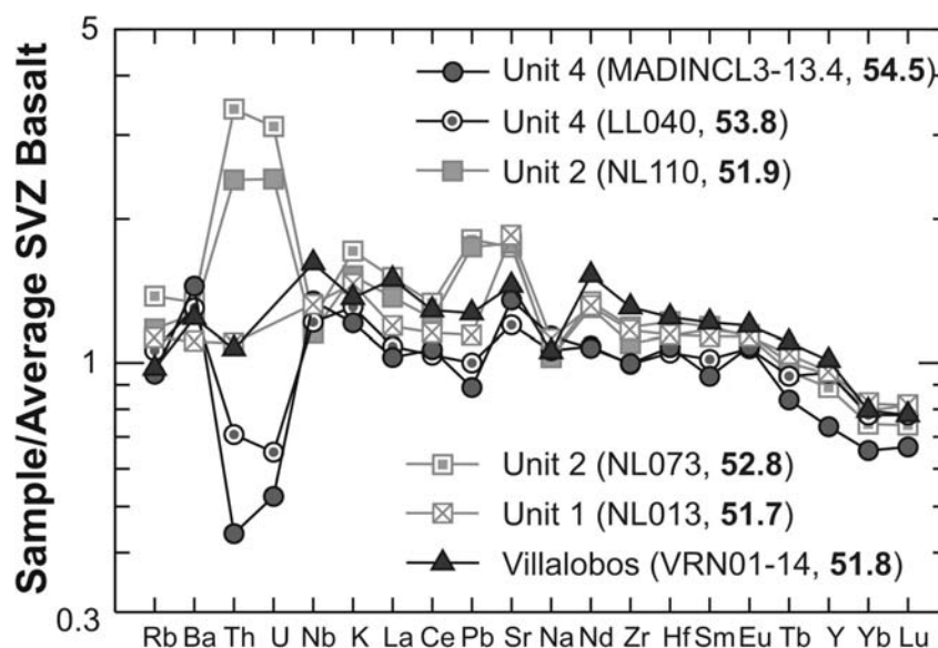
Figure 22. Multielement spidergram for selected mafic samples. In parenthesis are indicated sample code and SiO 2 content (in wt%, anhydrous basis). All analyses normalized to the average composition of ~30 SVZ basalts. Values used for normalization (in ppm) are Rb: 11.4, Ba: 166, Th: 1.3, U: 0.4, Nb: 2, K: 4317, La: 7.3, Ce: 18.1, Pb: 6.3, Sr: 432, Na: 22850, Nd: 10.9, Zr: 68, Hf: 1.8, Sm: 2.9, Eu: 0.97, Tb: 0.49, Y: 17, Yb: 1.8, Lu: 0.27.
