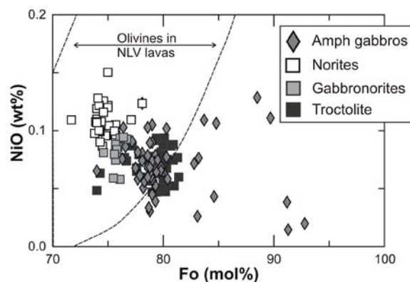
Figure 12. Fo-NiO composition of olivine crystals in xenoliths compared to the field of compositions in NLV lavas.
