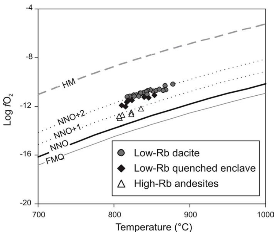
Figure 13: Temperature versus oxygen fugacity data from magnetite-ilmenite pairs calculated on the basis of the Andersen et al. (1993) algorithm. Oxygen fugacity buffers are FMQ= fayalite-magnetite-quartz; NNO= nickel-nickel oxide; HM= hematite-magnetite.
