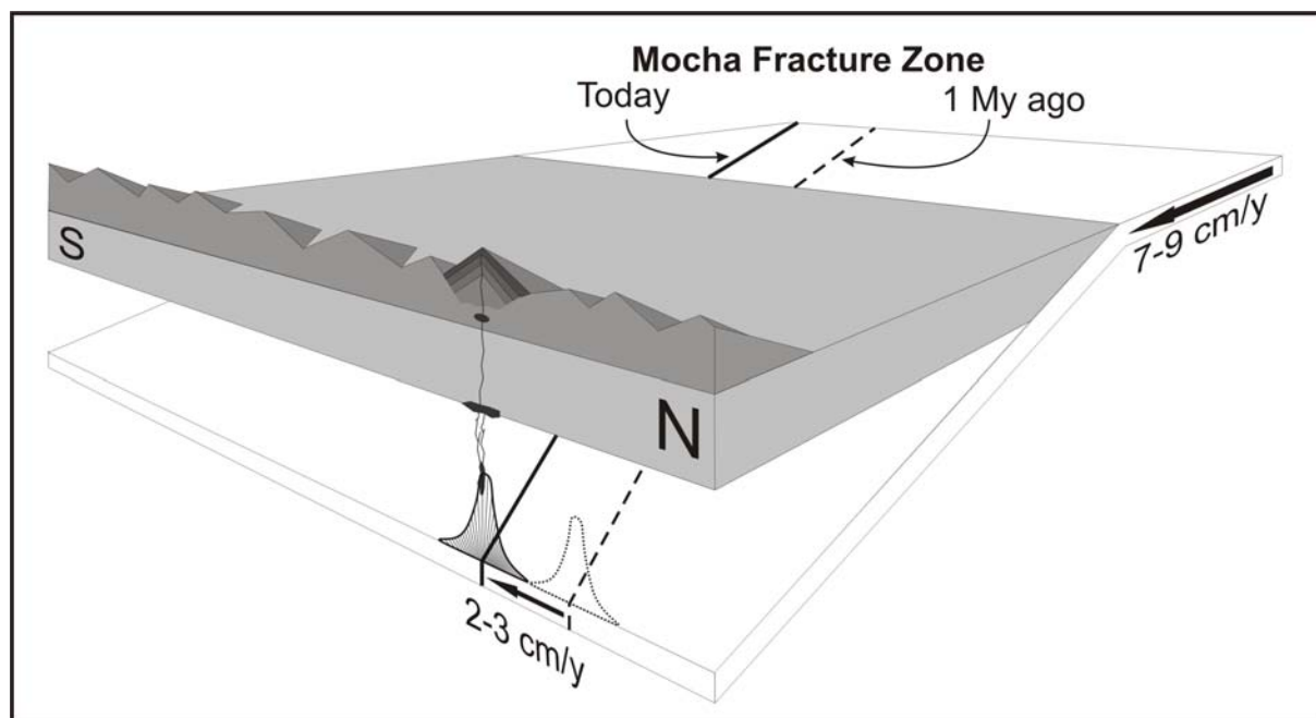
Figure 25. Schematic block-diagram of the southward-migrating Mocha fracture zone along the Southern Volcanic Zone.
