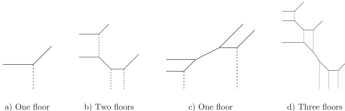
FIGURE 10. Floors of tropical curves
