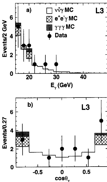
Fig. 1. (a) Distribution in energy of single-photon candidate events together with expectations based on Monte Carlo simulation of Standard Model processes. (b) The \cos\theta_\gamma spectrum of the single-photon candidates and Standard Model expectations.
