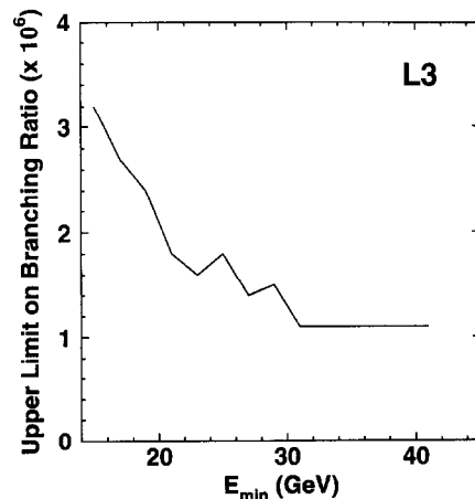
Fig. 4. Upper limit at the 95% C.L. on the branching ratio for Z decay to invisible particles and a photon with energy greater than E_{\min} . The limit has been calculated in steps of 2 GeV for E_{\min} .
