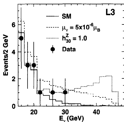
Fig. 2. The energy spectra of single-photon events expected in our search from (a) the Standard Model only (solid histogram), (b) the Standard Model modified to give the \tau neutrino a magnetic moment of the magnitude indicated (dashed histogram), and (c) the Standard Model extended to include an anomalous ZZγ coupling (dotted histogram). See text for additional description of models. The points show the energy spectrum of the single-photon candidates found in the search.
