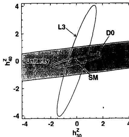
Fig. 3. Upper limits at the 95% C.L. on the ZZγ coupling parameters h_{30}^Z and h_{40}^Z obtained by L3 and by D0 [22] for \Lambda_Z = 500 GeV. The Standard Model prediction is indicated by the dot. The region of parameter space allowed by unitarity is shaded.
