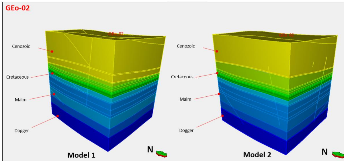
Figure 20 two different geological model (Model-1 and Model-2) developed for GGeo 2 arising from the two different structural model used as input.
