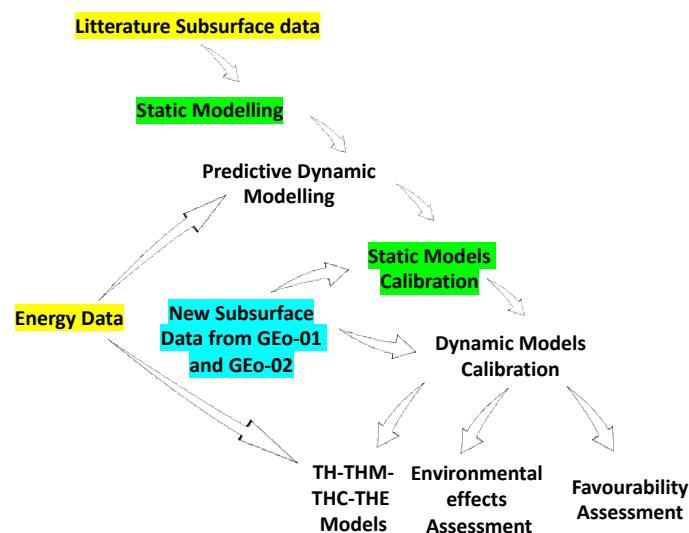
Figure 1 General workflow implemented in HEASTORE for HT-ATES potential assessment. Highlighted are the different phases involved in the static modelling activities
