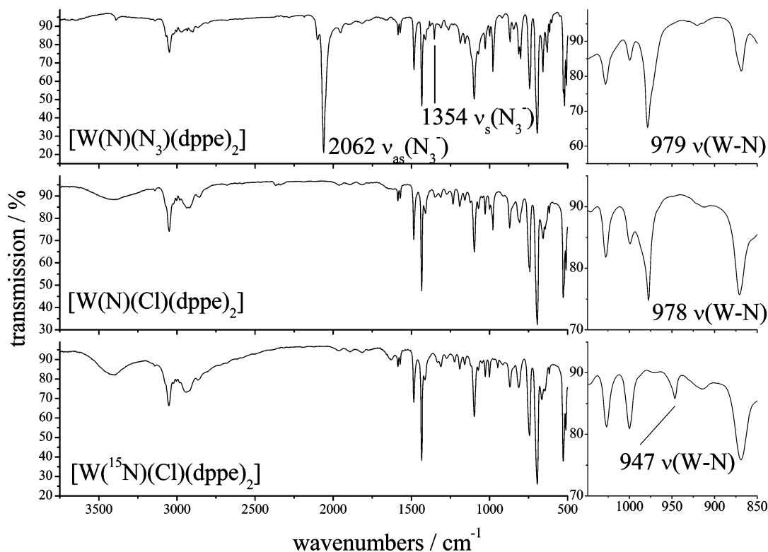
Figure 1. IR spectra of nitrido complexes [\text{W}(\text{N})(\text{N}_3)(\text{dppe})_2] ( 2 ), [\text{W}(\text{N})(\text{Cl})(\text{dppe})_2] ( 4 ), and [\text{W}(^{15}\text{N})(\text{Cl})(\text{dppe})_2] ( 4 ( ^{15}\text{N} )).
