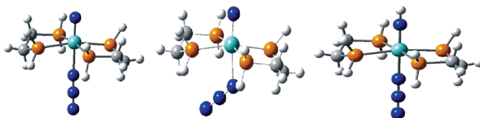
Figure 4. Geometry-optimized structures of [\text{Mo}(\text{N})(\text{N}_3)(\text{PH}_2\text{CH}_2\text{CH}_2\text{PH}_2)_2] ( I ) (left), I ( 3 E exc. st.) (middle), and [\text{Mo}(\text{NH})(\text{N}_3)(\text{PH}_2\text{CH}_2\text{CH}_2\text{PH}_2)_2]^+ ( I*H + ) (right).
