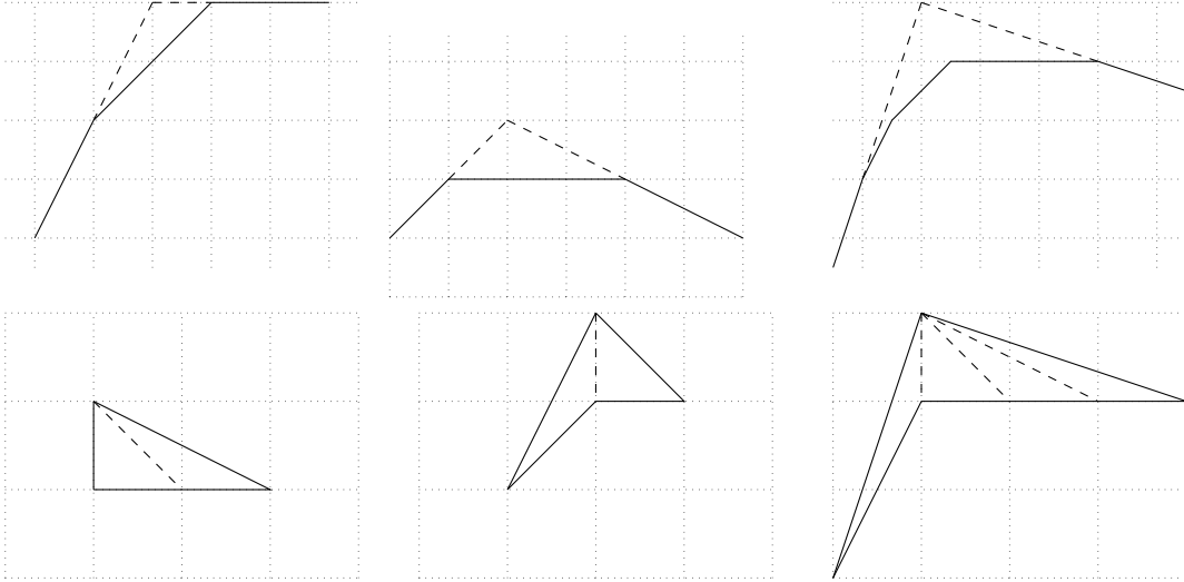
Figure 4.2: The canonical resolution of toric singularities can be extracted either from the dual cone or from the chain fraction for the slope of the corner.
