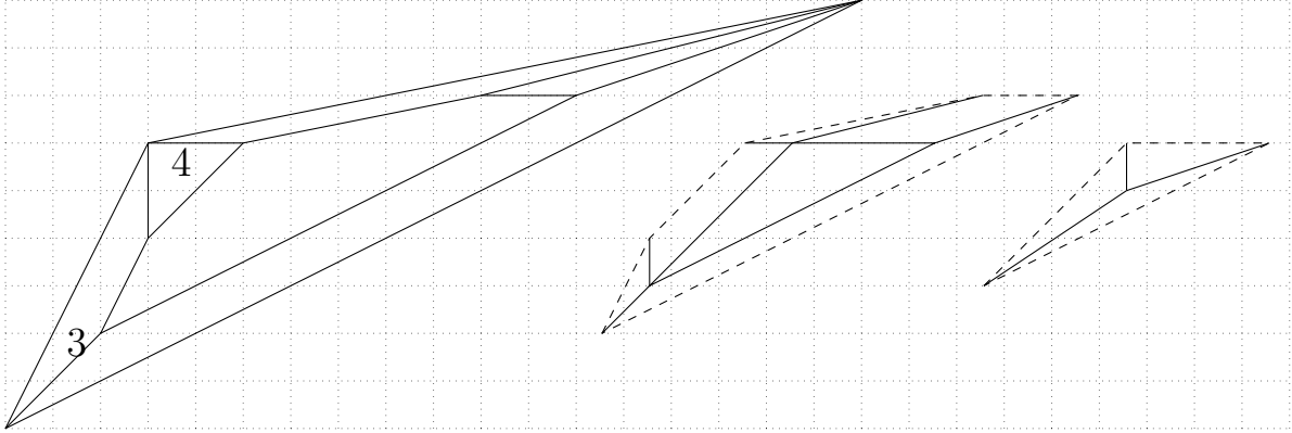
Figure 4.3: The evolution of triangle with no past (only the down left corner has exactly one adjacent edge of the curve) decomposed into three periods. The pentagon in the middle has three smooth corners and two singular, where the multiple edges go. Note that the level set of F_\omega near its maximum could have infinite past unless we didn't do so many blow-ups. The big triangle \Omega contains the whole information about the future — C_\Omega is the trajectory traced by the vertices of shrinking polygons.
