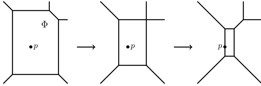
FIGURE 7. Illustration for Remark 4.34. The operator G_p shrinks the face \Phi where p belongs to. Firstly, t = 0 , then t = 0.5 , and finally t = 1 in \text{Add}_{ij}^{ct} f . Note that combinatorics of the new curve can change when t goes from 0 to 1.
