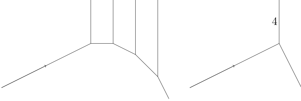
Figure 6.5: We go from the maximum (somewhere down left), accumulating degenerate branchings, when we do a branching right after a previous one, in the limit results in formation of a multiple edge. According to Figure 6.2, the multiplicity of the branching is equal to the multiplicity of the multiple edge stemming from it. Also compare to Figure 4.1, where the resolution is done in a specific example.
