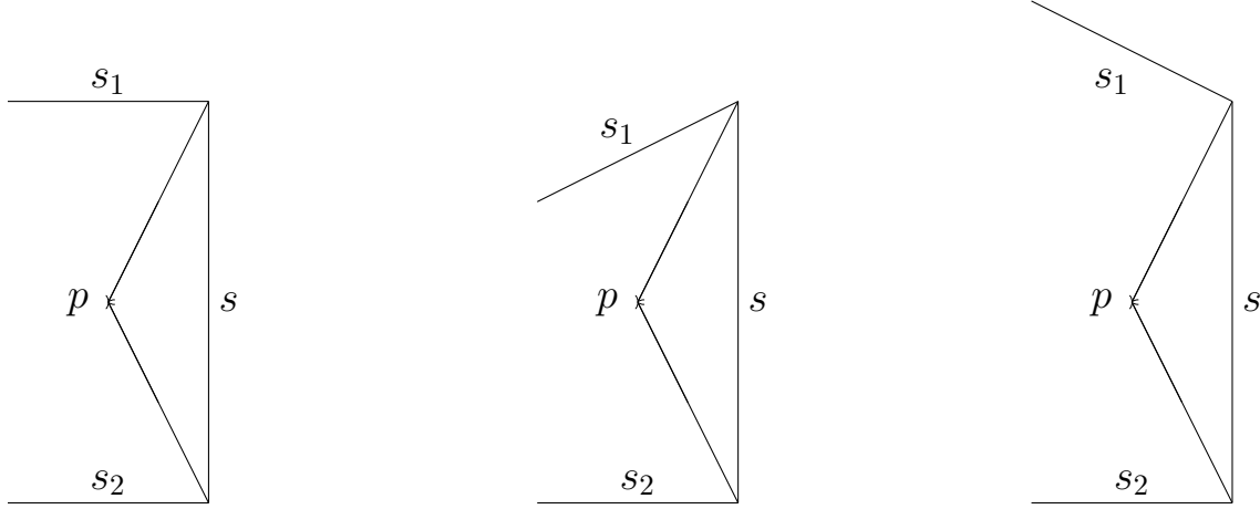
Figure 3.6: The possible configurations of sides with respect to a pair of collided particles. The collision happens at p to the left from the vertical side s . In the first case the adjacent sides s_1 and s_2 are parallel, in the second case their prolongations intersect to the left from s or to the right in the third case.
