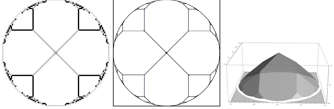
FIGURE 2. Additional grain of sand thrown to the center of \Omega = \{x^2 + y^2 \leq 1\} . The sand picture for h = 1/100 is on the left and the limit as h \rightarrow 0 is in the center. On the right we see the limit of the toppling function. Note that the central picture shows the corner locus of the right picture which is l_\Omega (Definition 4.3) for \Omega = \{x^2 + y^2 \leq 1\} .
