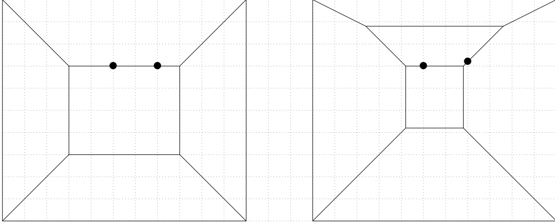
Figure 5.4: An unstable configuration and its perturbation (by a light shift of the right point) together with action minimising curves passing through them (solutions of Steiner problem). A wrong rounding at the sandpile approximation of the problem in similar cases produces globally observable, surviving in the thermodynamical limit, jumps in mass and action comparing to the expected tropical solution of the Steiner problem. We can modify the whole setup, making it sort of more realistic, using a concept of stable tropical intersection taking as the solution the limit of local perturbations, dissolving unstable energy in terms of sandpiles. Also the number of iterations of G_{p_1}G_{p_2} needed to arrive to the picture on the right actually gets tiger when the perturbation is small.
