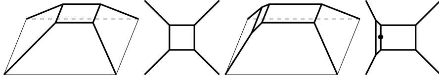
FIGURE 4. On the left: \Omega -tropical series \min(x, y, 1-x, 1-y, 1/3) and the corresponding tropical curve. On the right: the result of applying G_{(\frac{1}{5}, \frac{1}{2})} to the left picture. The new \Omega -tropical series is \min(x + \frac{2}{15}, y, 1-x, 1-y, \frac{1}{3}) and the corresponding tropical curve is presented on the right. The fat point is (\frac{1}{5}, \frac{1}{2}) .
