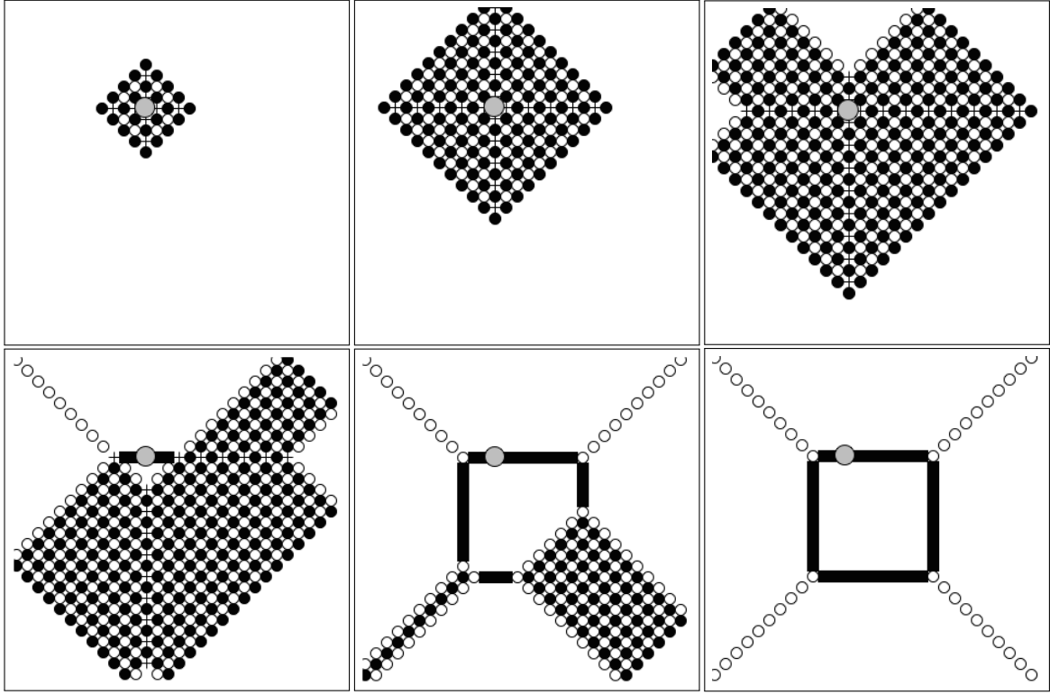
Figure 1.1: Snapshots during the relaxation for the state \phi \equiv 3 on a square after adding an extra grain at one point p (the big gray point). Black rounds represent v with \phi(v) \geq 4 , black squares (which are arranged along the vertical and horizontal edges on the final picture) represent the value of sand equal to 2, white rounds (arranged along diagonals on the final picture) are 1, and white cells are 3. Rare cells with zero grains are marked as crosses, one can see them during the relaxation on the vertical and horizontal lines through p . The value of the final state at p is 3.
