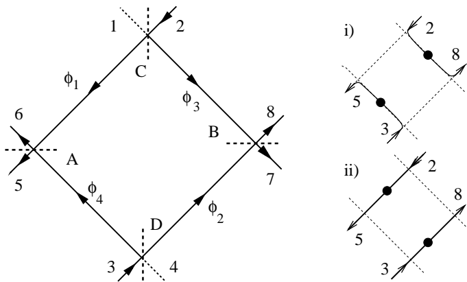
FIG. 1: Left: Two-source, four-detector optical Hanbury Brown Twiss geometry. Two beams, incident from 2 and 3 are split at the mirrors C and D and impinge on the mirrors A and B to reach detectors along the directions 5 to 8. Right: The two scattering processes i) and ii) contributing to the phase dependence of the correlators (see text).
