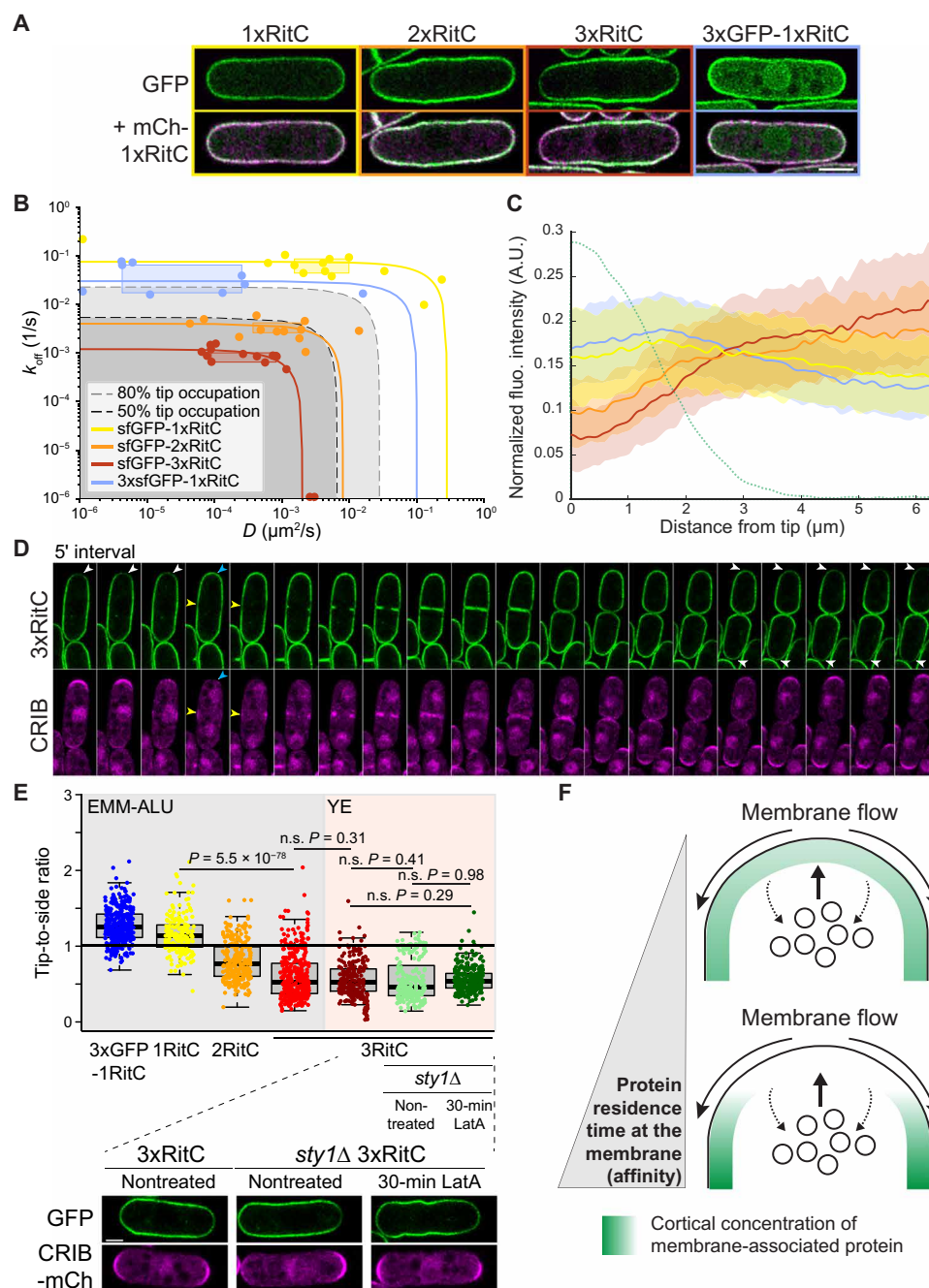
Fig. 4. The lateral diffusion and detachment rates of peripheral membrane proteins condition their cortical distribution by coupling to bulk membrane flows.
