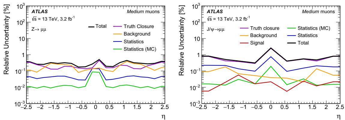
Fig. 1 Total uncertainty in the efficiency scale factor for Medium muons as a function of \eta as obtained from Z \rightarrow \mu\mu data (left) for muons with p_T > 10 GeV, and from J/\psi \rightarrow \mu\mu data (right) for muons with 5 < p_T < 20 GeV. The combined uncertainty is the sum in quadrature of the individual contributions
