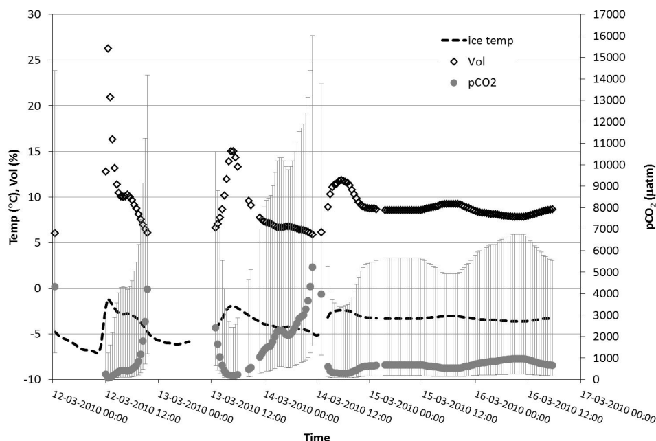
Fig. 5. Measured ice surface temperature (°C) and calculated brine volumes (%) and p\text{CO}_2 (µatm) in the brine channels from 12 to 16 March. The error bars around the p\text{CO}_2 are based on maximum and minimum values using the standard deviation on the measured salinity, TCO 2 and TA (see Table 1).
