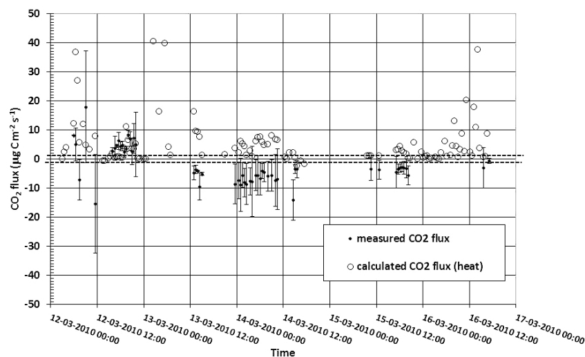
Fig. 8. The measured fluxes and the calculated fluxes using varying concentration based on brine volume calculated from ice temperature and R_c using the heat flux parameterization of R_c (○) as in Fig. 7. The CO 2 flux is estimated from EC technique, the cospectra peak method and the dissipation method. The dot shows the mean of the three methods and the bar shows the standard deviation.
