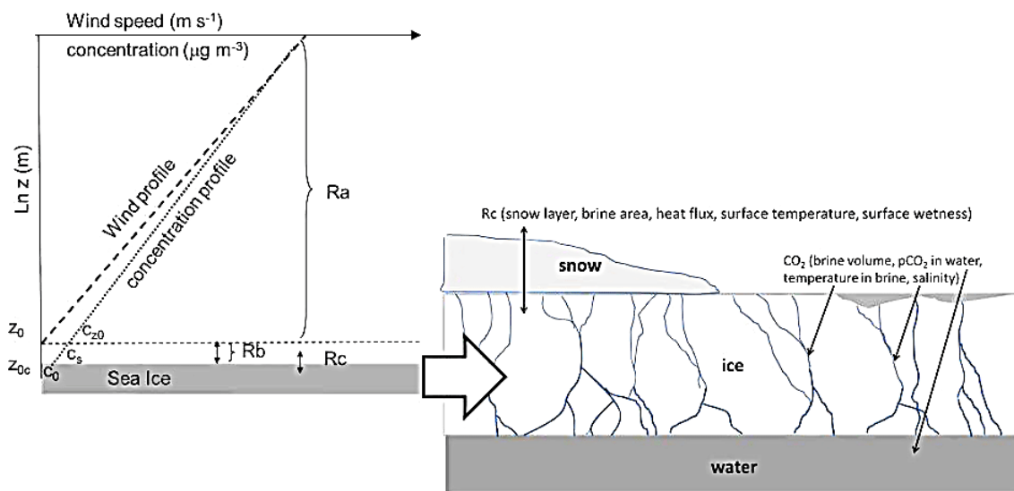
Fig. 1. Left panel: R_a is the aerodynamic resistance over the layer dominated by atmospheric turbulence. R_b is the quasi-laminar boundary layer resistance over the layer, which is influenced by molecular diffusion and turbulence and R_c is the resistance over the ice/snow–atmosphere interface. The dashed line illustrates the logarithmic wind profile over the surface, which in theory goes to 0 at z_0 . The dotted line illustrates the logarithmic concentration profile, which goes to the surface equilibrium concentration ( c_s ) at z_{0c} . Right panel: Sketch showing R_c and some of the parameters in/at the surface which R_c is affected by and p\text{CO}_2 in the brine and parameters affecting this.
