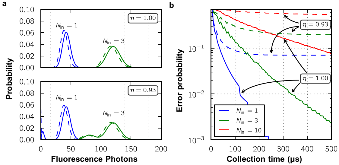
Figure 4. Estimation of the input photon number and the associated error probability. (a) Fluorescence photon number distribution for N_{\text{in}} = 1 and 3 input photons for a collection time of 150 \mu\text{s} . The upper plot shows the case of the ideal conversion efficiency. Dashed lines are without the contribution from the spontaneous decay of ions from the D_{5/2} state. Vertical dashed lines indicate the thresholds for photon number estimation. In the lower plot the finite conversion efficiency ( \eta = 0.93 ) leads to the possibility of estimating a photon number lower than N_{\text{in}} . (b) Probability of estimating a photon number different from N_{\text{in}} , for N_{\text{in}} = 1, 3 or 10. The error probability decreases with collection time, but has a lower limit for finite conversion efficiency.
