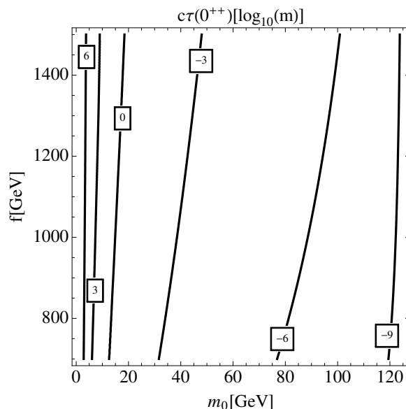
Figure 6. Decay length c\tau_0 of the G_{0+} state in \log_{10} (meters) as a function of m_0 and f .
