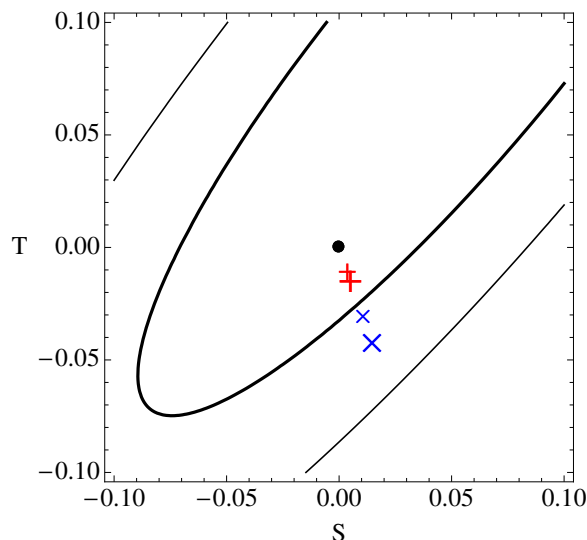
Figure 10. Close-up of the one- and two-sigma S, T ellipses marginalized over U with contributions from both the SM-like Higgs and the heavy twin Higgs \hat{h} . The small (large) blue “ \times ” shows the S, T prediction including a heavy twin Higgs of mass m_{\hat{h}} = 750 GeV (1.5 TeV) for f = 3v , while the small (large) red “ + ” shows the S, T prediction including a heavy twin Higgs of mass m_{\hat{h}} = 750 GeV (1.5 TeV) for f = 5v . The black dot denotes the contribution of a purely Standard Model Higgs of mass m_h = 125 GeV.
