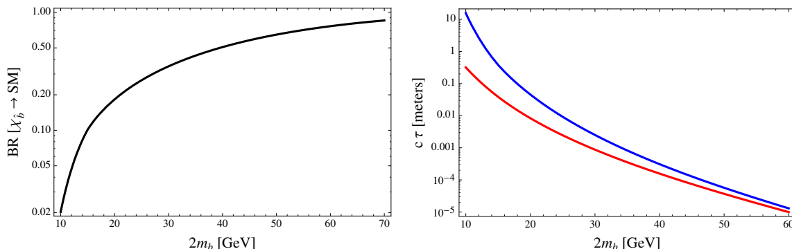
Figure 9. Features of \hat{\chi} decay; we emphasize that these results have very substantial uncertainties due to the limitations of our estimation methods. Left: branching ratios of \hat{\chi} into the SM along the BD-boundary line m_{G_{0+}} = m_{\hat{b}} , assuming twin neutrinos are massless. Right: decay length of \hat{\chi} for m_{G_{0+}} = m_{\hat{b}} , where the lower red (upper blue) curve refers to massless (heavy) twin neutrinos.
