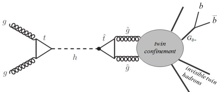
Figure 1. Example of a Twin Higgs collider event. The SM-like Higgs decays through a loop of the twin tops into a pair of twin gluons, which subsequently hadronize to produce various twin glueballs. While some glueballs are stable at the collider scale, G_{0+} decay to Standard Model particles is sufficiently fast to give LHC-observable effects, including possible displaced vertices. The h\hat{g}\hat{g} coupling, indicated by a black dot, is generated by small mixing of the Higgs and the twin Higgs.
