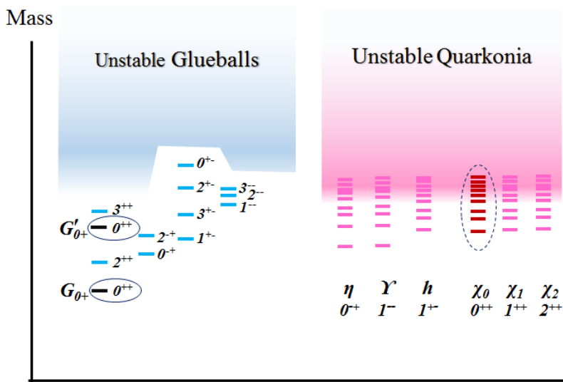
Figure 4. Sketch of the twin hadron spectrum in the regime where m_0 < 2m_{\hat{b}} < 2m_0 . In addition to the G_{0^+} , of mass m_0 , about a dozen other glueballs, with mass splittings of order m_0 , are stable against twin strong decays. Numerous twin bottomonium states, including a tower of 0^{++} states \hat{\chi} , are stable against twin strong decays. The circled G_{0^+} and G'_{0^+} glueballs, and potentially the \hat{\chi} quarkonia, can dominantly decay via annihilation through an s -channel off-shell Higgs to the SM.
