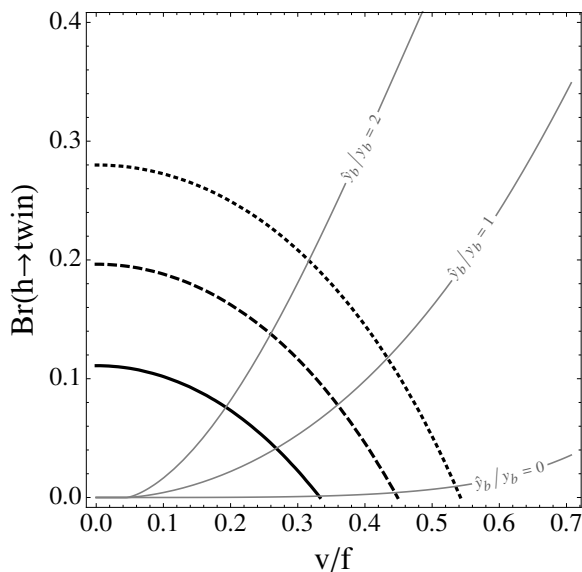
Figure 8. Current bounds on v/f and the Higgs branching ratio into the twin sector from a combined fit to Higgs coupling measurements. Solid, dashed, and dotted black lines denote the 1-, 2-, and 3- \sigma bounds (defined as \Delta\chi^2 = 2.30, 6.18, 11.83 ) due to ATLAS and CMS Higgs coupling measurements. The grey lines correspond to the perturbative calculation of the Higgs branching ratio into the twin sector as a function of v/f for \hat{y}_b/y_b = 0, 1, 2 ; as discussed in the text, the actual branching ratio may differ significantly from the perturbative result for a given value of \hat{y}_b .
