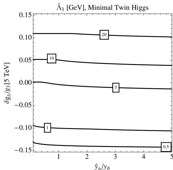
Figure 3. The confinement scale \hat{\Lambda}_3 of the twin SU(3) coupling given fractional variations in \hat{g}_3 and \hat{y}_b at the cutoff \Lambda for the minimal Twin Higgs (dependence on \hat{y}_t is negligible). Here we take \Lambda = 10\hat{m}_t and f = 3v . The mild kinks are due to the \hat{b} threshold.
