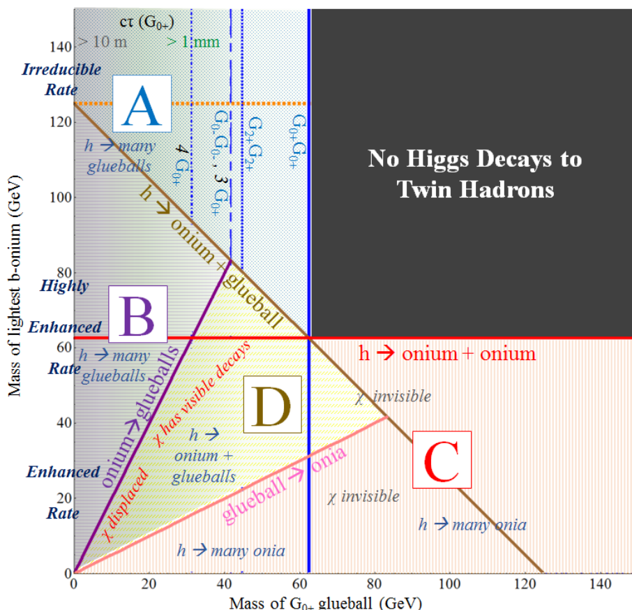
Figure 7. A qualitative overview of the phenomenology, for f = 3v , in the various regions of parameter space; see figure 5. Details are explained in subsequent sections. Solid lines indicate kinematic boundaries. Common final states are indicated in italics. At low glueball mass, decays of the G_{0+} are displaced; see figure 6. Here it is assumed that there are light twin leptons, so one \hat{\chi} state is visible, and even displaced, only in small regions; otherwise \hat{\chi} decays visibly throughout regions C and D, and is displaced at low mass.
