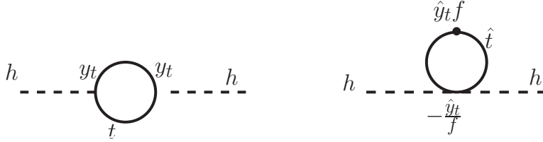
Figure 2. Cancellation of the top divergence in the Twin Higgs model. The effective vertex in the second diagram arises upon integrating out the heavy radial mode.
