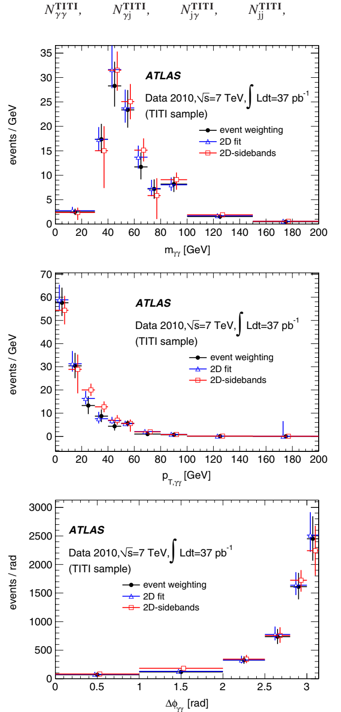
FIG. 3 (color online). Differential \gamma\gamma yields in the TITI sample ( N_{\gamma\gamma}^{\text{TITI}} ), as a function of the three observables m_{\gamma\gamma} , p_{T,\gamma\gamma} , \Delta\phi_{\gamma\gamma} , obtained with the three methods. In each bin, the yield is divided by the bin width. The vertical error bars display the total errors, accounting for both the statistical uncertainties and the systematic effects. The points are artificially shifted horizontally, to better display the three results.
