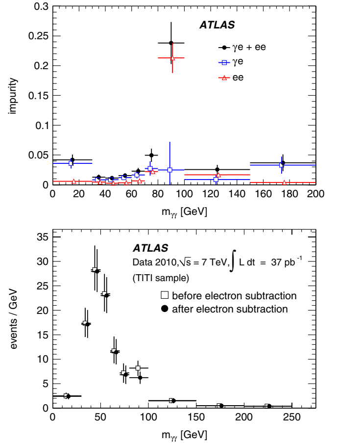
FIG. 6 (color online). Electron background subtraction as a function of m_{\gamma\gamma} . The top plot displays the impurity, overall and for the \gamma e and ee separately. The bottom plot shows the di-photon yield before (open squares) and after (solid circles) the electron background subtraction. The points are artificially shifted horizontally, to better display the different values.
