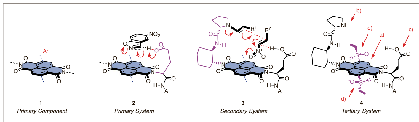
Fig. 2. Covalent coupled systems: A \pi -acidic aromatic surface 1 as primary component (blue; primary function: anion binding) is interfaced with a carboxylate to give primary system 2 (emergent property: catalysis of Kemp elimination (red arrows), an amine for secondary system 3 (emergent property: catalysis of enamine addition) and sulfoxides for tertiary system 4 (emergent property: stereoselectivity) with four distinct, covalently interfaced components contributing to function (a-d). Compare Fig. 3 for explicit systems analysis.
