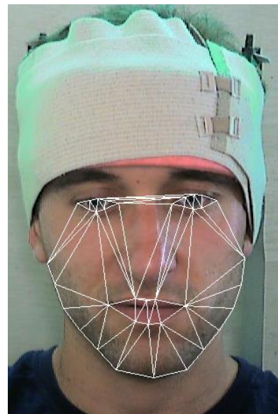
Figure 9 Delaunay triangulation
