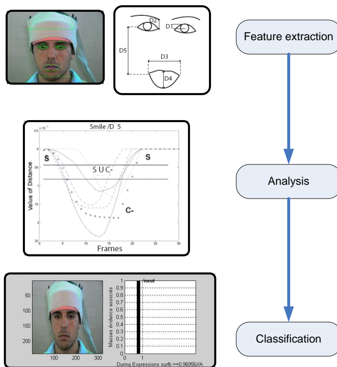
Figure 6 Illustration of the feature extraction, analysis and classification system for emotion detection.
