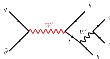
Fig. 1. Feynman diagram for W' -boson production with decay into t\bar{b} and a hadronically decaying top quark.
