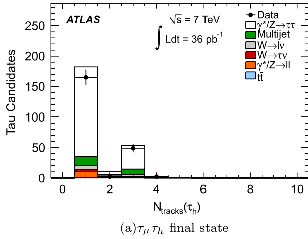
FIG. 5 (color online). Distribution of the number of tracks associated to \tau candidates after the full selection, including the opposite-charge requirement for the \tau candidate and the lepton, except the requirement on the number of tracks and on the magnitude of the \tau charge.
