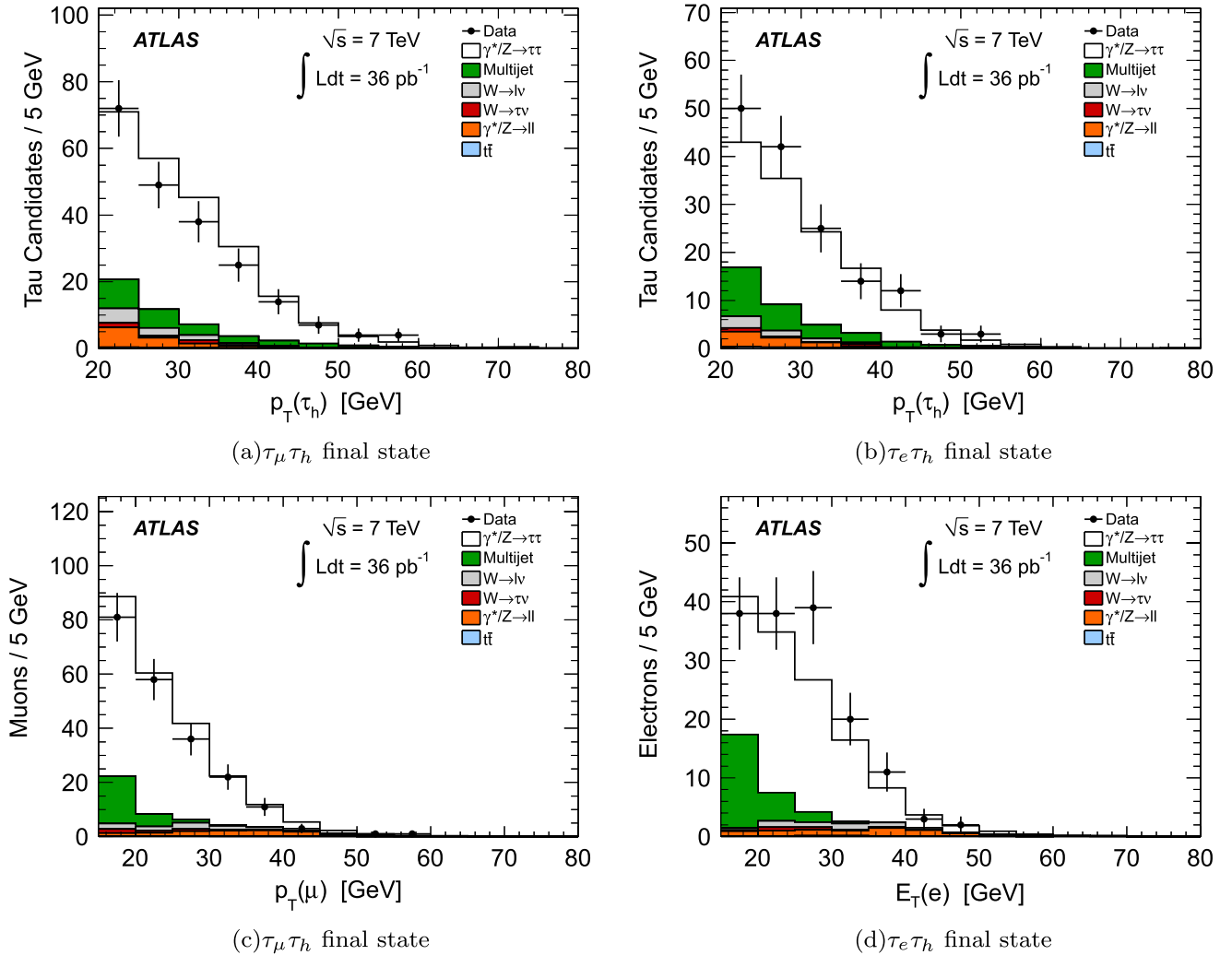
FIG. 4 (color online). Distributions of the p_T of the \tau candidate and of the muon and E_T of the electron, for events passing all signal selections for the \tau_\mu \tau_h and \tau_e \tau_h final states.
