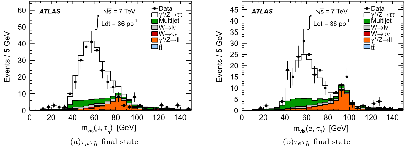
FIG. 3 (color online). The distributions of the visible mass of the combination of the \tau candidate and the lepton are shown for the (a) \tau_\mu \tau_h and (b) \tau_e \tau_h final states. These distributions are shown after the full event selection, except for the visible mass window requirement.
