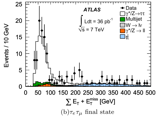
FIG. 6 (color online). Distributions of the variables (a) \sum \cos\Delta\phi , after the lepton isolation selection and (b) \sum E_T + E_T^{\text{miss}} after the \sum \cos\Delta\phi selection, for the \tau_e \tau_\mu final state. The multijet background is estimated from data according to the method described in Sec. V; all other processes are estimated using MC simulations.
