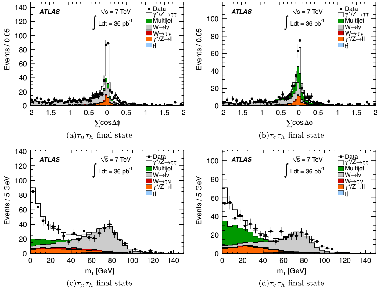
FIG. 2 (color online). The distributions of \sum \cos \Delta \phi are shown for the (a) \tau_\mu \tau_h and (b) \tau_e \tau_h final states. The distributions of the transverse mass, m_T , are shown for the (c) \tau_\mu \tau_h and (d) \tau_e \tau_h final states. All distributions are shown after the object selection for the given final state and after requiring exactly one muon or electron candidate. A requirement on the charge of the \tau candidate to be of opposite sign to that of the lepton is also applied. The multijet background is estimated from data according to the method described in Sec. V; all other processes are estimated using MC simulations.
