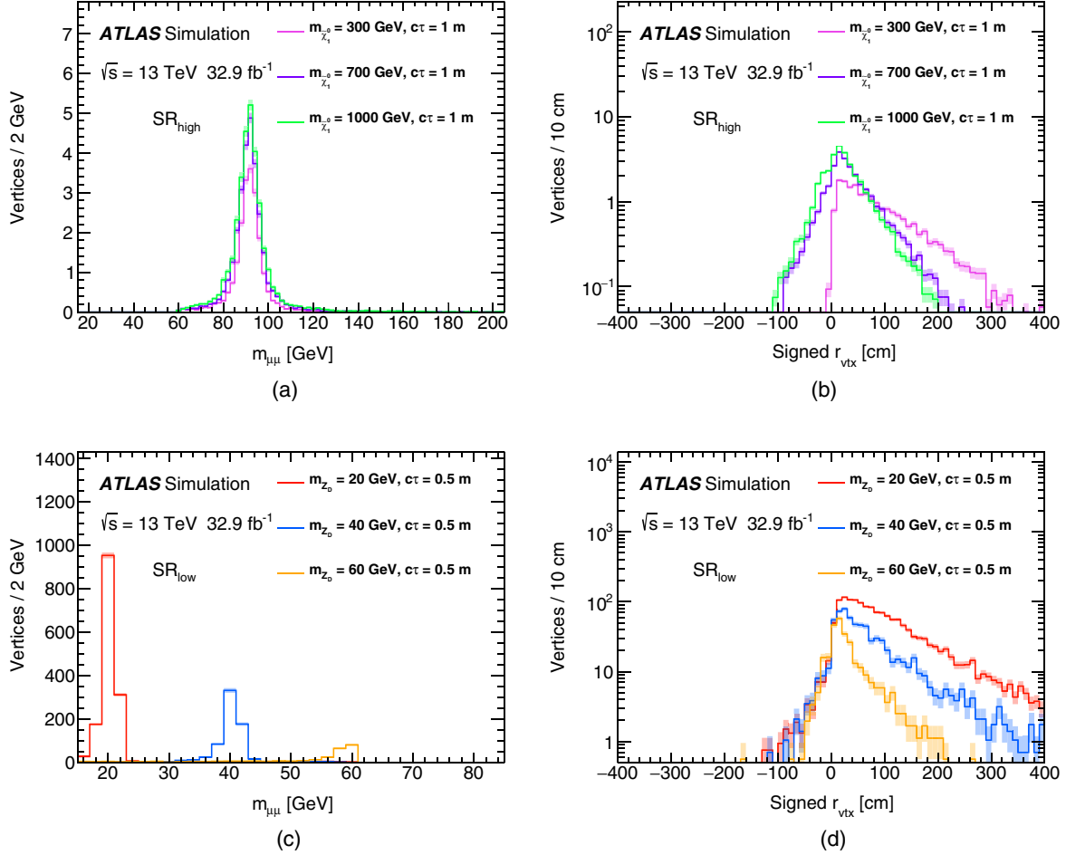
FIG. 5. Distributions derived from MC simulations of (a) dimuon invariant mass m_{\mu\mu} and (b) vertex radius r_{vtx} for signal vertices in SR_{high} with a long-lived neutralino, \tilde{\chi}_1^0 ( m_{\tilde{\chi}_1^0} = 300, 700 , and 1000 GeV and c\tau_{\tilde{\chi}_1^0} = 100 cm) decaying to a Z boson (with Z \rightarrow \mu^+\mu^- ) and a gravitino; (c) m_{\mu\mu} and (d) r_{vtx} for signal vertices in SR_{low} with a long-lived dark photon, Z_D ( m_{Z_D} = 20, 40 , and 60 GeV; and c\tau_{Z_D} = 50 cm), that decays to \mu^+\mu^- . The shaded bands represent the statistical uncertainties. The distributions are normalized to the expected yields in the signal regions for m_{\tilde{g}} = 1100 GeV, \sigma(pp \rightarrow \tilde{g}\tilde{g}) = 0.1635 pb, B(\tilde{\chi}_1^0 \rightarrow Z\tilde{G}) = 1.0 , and B(Z \rightarrow \mu^+\mu^-) = 0.03366 ; and m_H = 125 GeV, m_{H_D} = 300 GeV, \sigma(pp \rightarrow H) = 44.1 pb, B(H \rightarrow Z_D Z_D) = 100\% , and the value of B(Z_D \rightarrow \mu^+\mu^-) varying between 0.1475 and 0.1066 for the range m_{Z_D} = 20 – 60 GeV.
