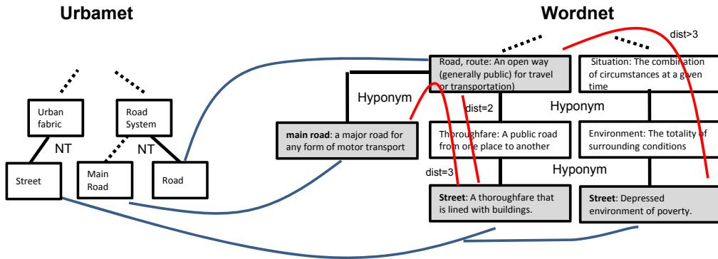
Figure 3: Example of context based disambiguation
