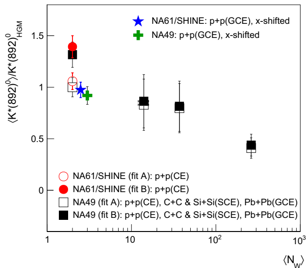
Fig. 15 The mean multiplicity of K^*(892)^0 for p+p reactions (this analysis and NA49 measurement [4]), as well as results of NA49 for C+C, Si+Si and Pb+Pb [4] interactions at 158A GeV/c divided by the HGM predictions [41] for fit B (closed circle and closed squares) and fit A (open circle and open squares), see the text for details. Closed star and cross symbols show p+p measurements compared to HGM predictions for the Grand Canonical Ensemble formulation [42,43]. N_w denotes the number of wounded nucleons taken from Ref. [4]
