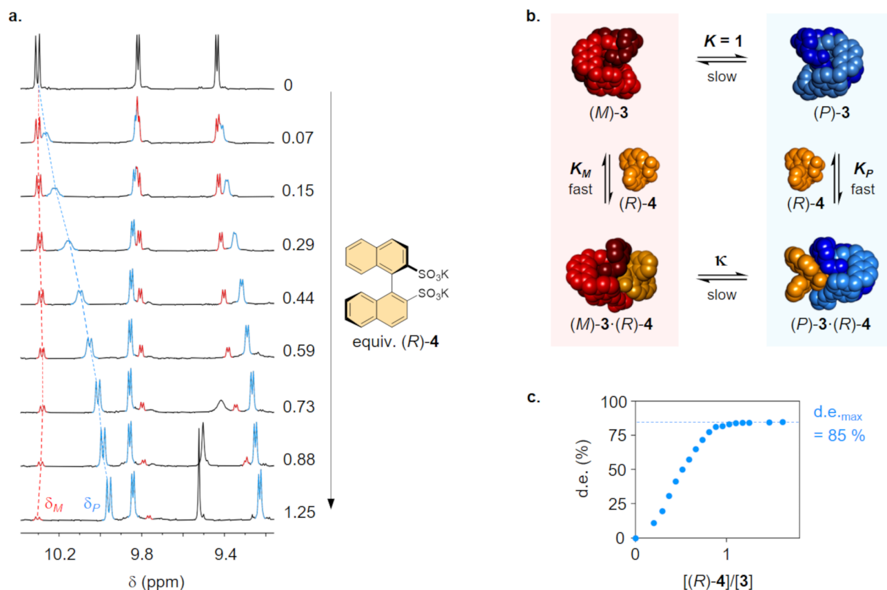
Figure 5. Amplification of the diastereomeric complex (P)\text{-}3 \cdot (R)\text{-}4 . (a) ^1\text{H} NMR titration of (R)\text{-}4 to a solution of [2]catenane 3 (1.13 mM, \text{D}_2\text{O}/\text{CD}_3\text{CN} 1:1, 500 MHz, 298 K). (b) Representation of the equilibria involved in the diastereoselective amplification. (c) Evolution of the diastereomeric excess in the course of the titration.
