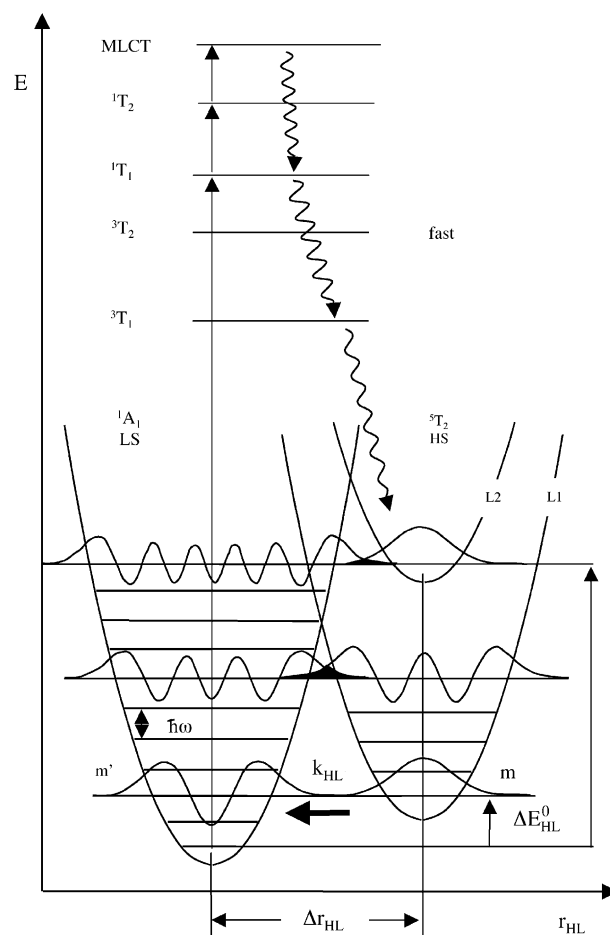
Fig. 1. The electronic structure of iron(II) spin-crossover (ligand L1) and low-spin complexes (ligand L2). The mechanisms for the light-induced population of the high-spin state following excitation into ligand-field or MLCT bands of the low-spin species are indicated by curly arrows. At low temperatures the barrier effectively traps the complex in the high-spin state. Potential wells of the high-spin and the low-spin state are shown along the totally symmetric normal coordinate. At low temperatures tunnelling occurs exclusively from the lowest vibrational state of the high-spin state. At elevated temperatures, tunnelling occurs as an activated process from thermally populated vibrational levels of the high-spin state. The zero-point energy difference \Delta E_{\text{HL}}^0 can be tuned chemically and physically.
