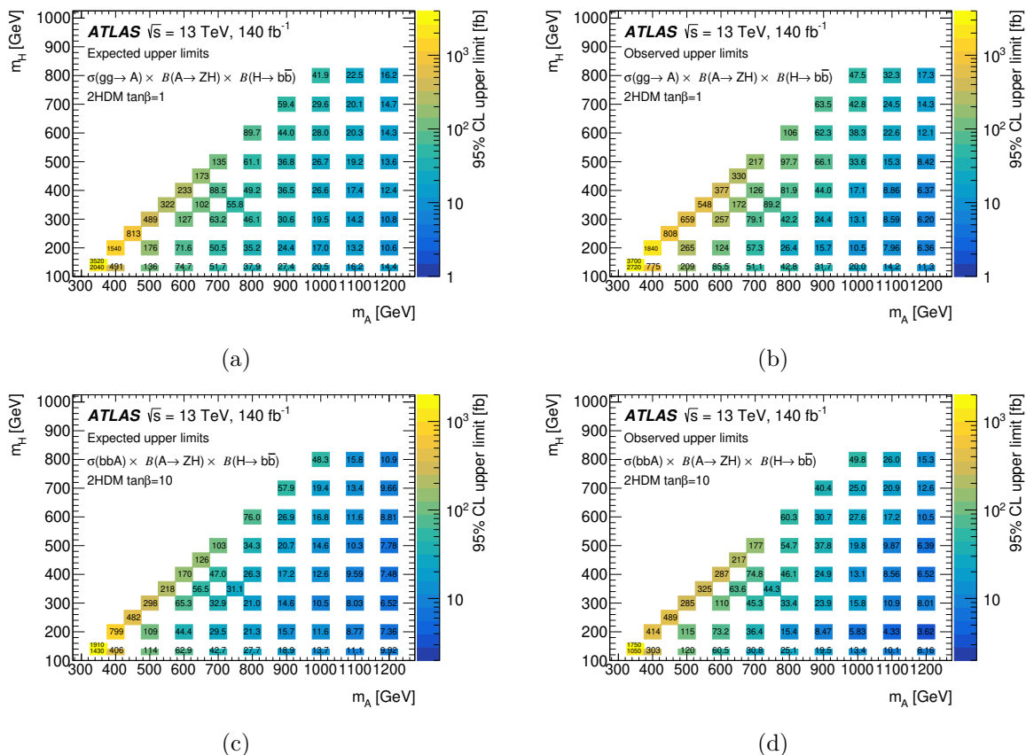
Figure 6. Expected (a,c) and observed (b,d) upper limits at 95% CL on \sigma(gg \rightarrow A) \times B(A \rightarrow ZH) \times B(H \rightarrow b\bar{b}) (a,b) and \sigma(bbA) \times B(A \rightarrow ZH) \times B(H \rightarrow b\bar{b}) (c,d) in the (m_A, m_H) plane. The limits are shown for either \tan \beta = 1 or \tan \beta = 10 in ggF or bbA production, respectively. The \tan \beta value is relevant only for the choice of A boson width.
