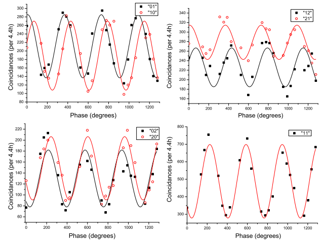
FIG. 8: Measured coincidence counts as a function of phase. Top-Left : BSA-results '01', '10'. Top-Right : BSA-results '12', '21'. Bottom-Left : BSA-results '02' and '20'. Bottom-Right : BSA-results '11'. Note that for each graph there is an unknown, but equal, offset of the phase-value.
