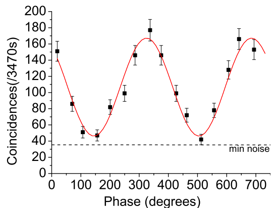
FIG. 7: The Result of the 1-Bell state teleportation experiment (a beamsplitter instead of the interferometer) with F_{raw} = 0.79 \pm 0.02 and F_{net} = 0.91 \pm 0.02 .
