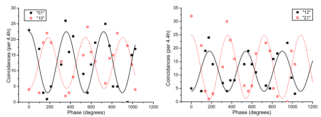
FIG. 11: Measurements of the Noise for a interferometer-BSA teleportation experiment. Left : ‘01’ and ‘10’ are in antiphase as expected and have Visibilities of V_{01} = 0.77 \pm 0.12 , V_{10} = 0.65 \pm 0.12 Right : ‘12’ and ‘21’ have a \pi phaseshift as expected and have Visibilities of V_{12} = 0.66 \pm 0.14 , V_{21} = 0.91 \pm 0.13
