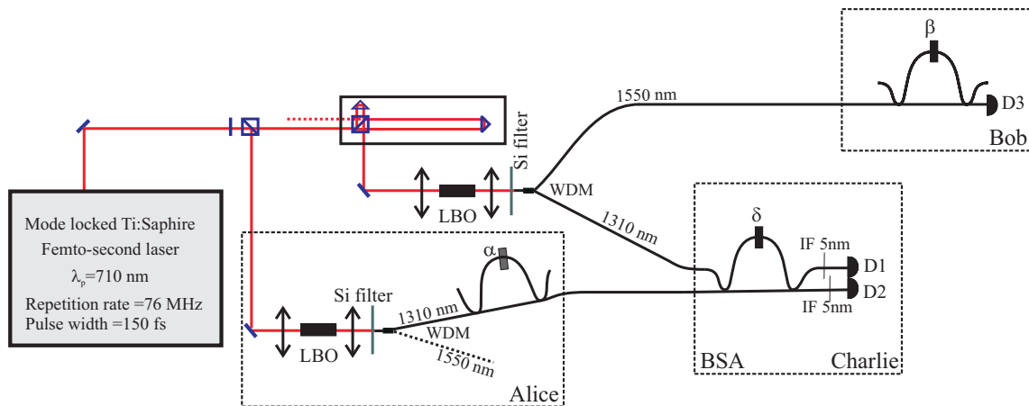
FIG. 3: A rough overview of the experimental setup. The fiber interferometers shown here are in reality Michelson-interferometers, for the interferometer in the BSA two circulators are used to have two separate inputs and outputs. Not shown in the figure is the method used for stabilizing the interferometers.
