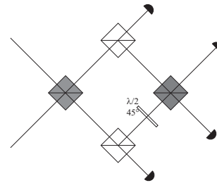
FIG. 2: A schematic representation of the new type of Bell-state Analyzer for polarization qubits. The grey cubes represent non-polarizing beamsplitters and the white cubes are polarizing beamsplitters.
