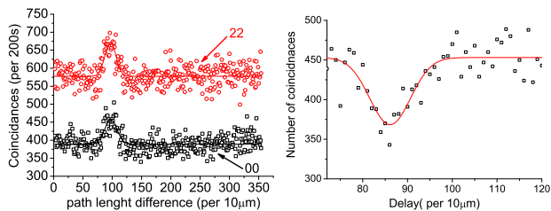
FIG. 5: Left, IF-BSA : Graph showing the number of measured coincidences as a function of a change in the delayline. Both ‘00’ and ‘22’ clearly show an anticrossing at the same location. The net visibilities are V_{00} = 32 \pm 3\% and V_{22} = 26 \pm 2\% Right, BS-BSA : Graph showing the decrease in the number of measured coincidences ‘00’ as a function of a change in the delayline [27]. The net visibility is V = 29 \pm 3\% .
