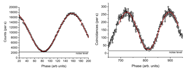
FIG. 4: Left : Single photon interference with V_{net} = 0.97 \pm 0.01 . Right : Franson-type Bell-test with V_{net} = 0.94 \pm 0.01 .
