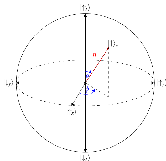
Fig. 7.6 The Bloch Sphere representation of a spin- \frac{1}{2} particle.
