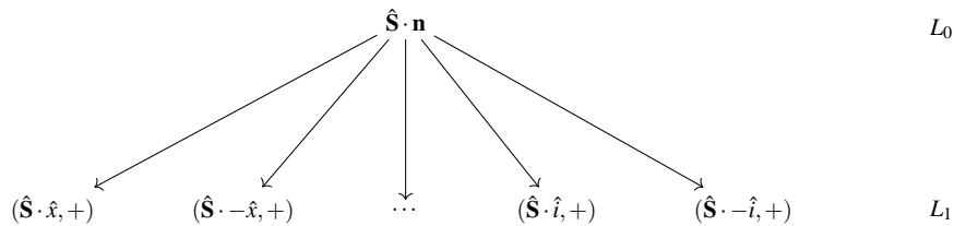
Fig. 7.7 Pictorial of Component Antirealism Spin Determinable Monism for spin- \frac{1}{2} systems. The maximally unspecific determinable is ‘having spin- \frac{1}{2} ’ at level L_0 represented by operator \hat{S} \cdot \mathbf{n} . Its determinates at L_1 are the particular directions along which the system’s spin could be polarised that we obtain by substituting \mathbf{n} with a precise spatial direction. Spin up and down along the x -axis, respectively, (\hat{S} \cdot \hat{x}, +) and (\hat{S} \cdot -\hat{x}, +) , are portrayed in the pictorial as an example. The dots indicate that the number of determinates is infinite. The maximally specific determinates (\hat{S} \cdot \hat{i}, +) and (\hat{S} \cdot -\hat{i}, +) , for a generic axis i , indicates that there are only two possible spin orientations for every axis. There is no further level of determination between the maximally unspecific determinable and its maximally specific determinates.
