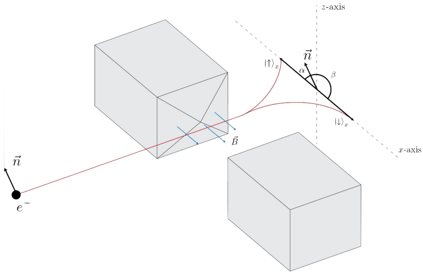
Fig. 7.8 Pictorial of a particle with polarization vector \mathbf{n} passing through a Stern-Gerlach magnet aligned along the x -axis.
