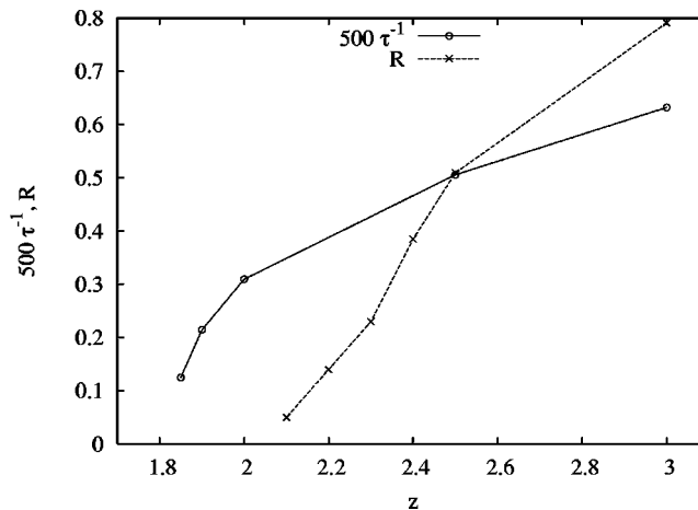
FIG. 2. The inverse average time between extinctions \tau^{-1} and the percolation probability R as a function of z . Plotted results are based on calculations for N=100, 200, 300, and 400 and extrapolation N \rightarrow \infty .
