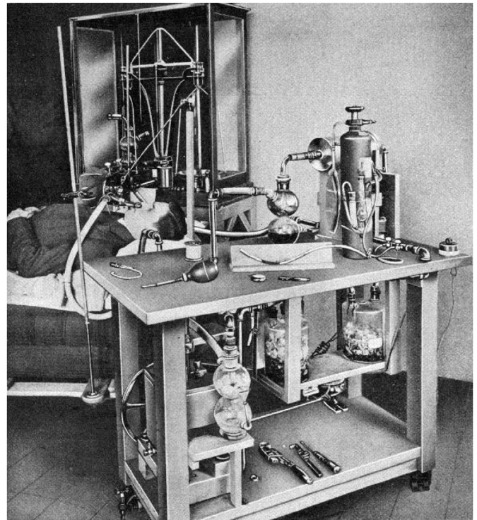
Fig. 1. The apparatus used by Benedict [3]. Reproduced with permission from the publishers.
