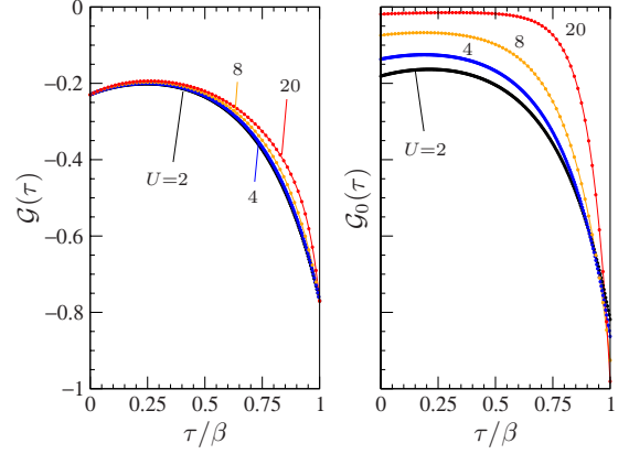
FIG. 10. (Color online) DMFT imaginary-time propagators calculated at \beta=1 and n=1.54 for various interaction strengths. The symbols show the QMC results on the discrete-time mesh. The solid lines are the fit, Eq. (B1), used to evaluate the self-energy shown in Fig. 4.
