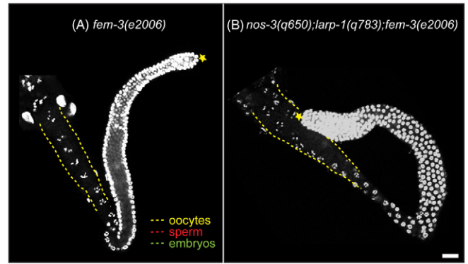
Fig. 4. larp-1 and nos-3 promote oogenesis in a fem-3 -dependent manner. Adult hermaphrodite germlines of the indicated genotypes were dissected and stained with DAPI. Approximately 95% of fem-3(e2006) (A) as well as nos-3(q650);larp-1(q783);fem-3(e2006) (B) hermaphrodite germlines are feminized (see also Table 1). Yellow star indicates the distal tip of the germline and dashed lines highlight sperm (red), oocytes (yellow) and embryos (green). Scale bar: 50 \mu m.
