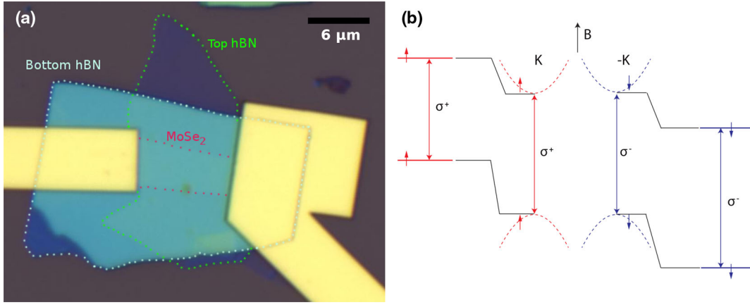
FIG. 1. A gate controlled MoSe 2 /h-BN heterostructure under external magnetic field. (a), The sample consists of a 9 \mu\text{m} by 4 \mu\text{m} MoSe 2 monolayer sandwiched between two h-BN layers. Gate voltage applied between the gold contacts to the MoSe 2 layer and the highly doped Si substrate allows for controlling the electron density in the monolayer. (b) The single particle picture of conduction and valence band shifts under a magnetic field B_z applied perpendicular to the plane of MoSe 2 . Assuming a large spin-orbit splitting, only the lowest (highest) energy conduction (valence) band is depicted. For B_z > 0 , the exciton resonance in the K valley redshifts along with the conduction band minimum in the -K valley. This opposite sign of the effective g factor of the excitons and electrons plays a key role in determining the absorption spectrum of MoSe 2 monolayers.
