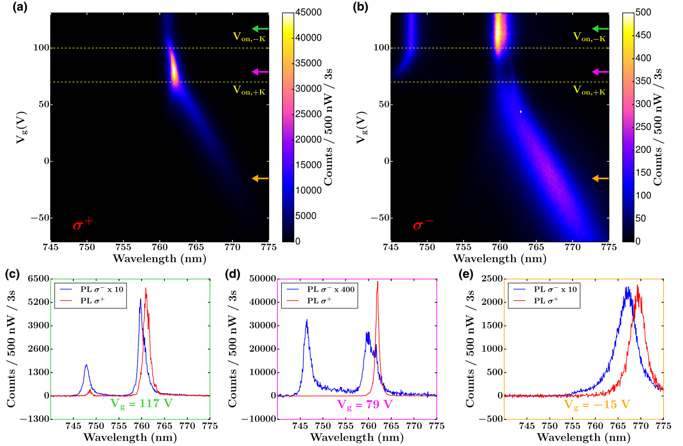
FIG. 2. Gate voltage dependent photoluminescence spectrum under a magnetic field of B_z = 7 T. (a) Gate voltage ( V_g ) dependent right-hand circularly polarized ( \sigma^+ ) photoluminescence (PL) spectrum of a \text{MoSe}_2/\text{h-BN} heterostructure at B_z = 7 T under excitation by a linearly polarized 719 nm laser. The depicted V_g axis is shifted by 10 V to compensate for the hysteretic behavior we observe in the gate scans (see Supplemental Material [26]). (b) The corresponding PL spectrum for left-hand circularly polarized ( \sigma^- ). (c) The line cut through the \sigma^+ and \sigma^- PL spectra at V_g = 117 V > V_{\text{on},-K} show that the PL exhibits a sizable degree of polarization where the ratio of \sigma^+ and \sigma^- polarized PL intensities is \approx 11 . (d) The line cut through the \sigma^+ and \sigma^- PL spectra at V_g = 79 V shows that the degree of PL polarization increases dramatically to yield a ratio of \sigma^+ and \sigma^- polarized PL intensities \approx 700 . (e) The line cut through the \sigma^+ and \sigma^- PL spectra at V_g = -15 V where both valleys have high n_e . The ratio of the right- ( \sigma^+ ) and left- ( \sigma^- ) hand circularly polarized PL intensities is reduced back to \approx 11 .
