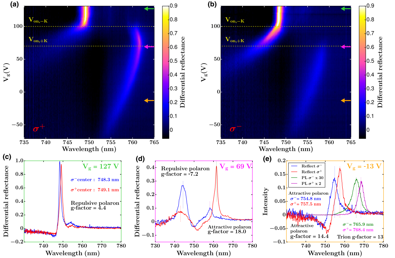
FIG. 3. Polarization resolved reflection spectrum under a magnetic field of B_z = 7 T. (a) Gate voltage ( V_g ) dependent right-hand circularly polarized ( \sigma^+ ) white light reflection spectrum of the \text{MoSe}_2/h\text{-BN} heterostructure at a magnetic field of B_z = 7 T. For V_g \leq V_{on,-K} = 100 V (yellow dashed horizontal line), we observe a blueshift of the exciton resonance whereas the strength of the attractive polaron resonance increases as it redshifts. (b) Reflection spectrum as in (a) but now for left-hand circularly polarized ( \sigma^- ) light. Only for V_g \leq V_{on,K} = 70 V, oscillator strength transfer to the attractive polaron is observed. Whereas the exciton oscillator strengths of the \sigma^+ and \sigma^- transitions for V_g > V_{on,-K} are nearly identical, the \sigma^+ attractive polaron is much stronger than its \sigma^- counterpart for V_{on,K} < V_g < V_{on,-K} . (c) The differential reflection spectrum of both \sigma^+ and \sigma^- light at V_g = 127 V: the two resonances have nearly identical shape and strength but their energies differ by 1.8 meV, yielding a g factor of 4.4. (d) The differential reflection spectrum as in (c) but now at V_g = 69 V: the splitting between the attractive polaron resonances is 7.3 meV, which corresponds to a g factor of \approx 18 . The \sigma^+ exciton or repulsive polaron energy on the other hand is lower than that of \sigma^- by \approx 2.9 meV, yielding a g factor of -7.2 . These results demonstrate that exciton-electron interactions strongly modify the magneto-optical response of \text{MoSe}_2 monolayers. (e) The differential reflection as well as PL spectrum of both \sigma^+ and \sigma^- light at V_g = -13 V.
