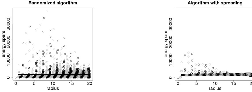
Figure 3: Simulations
