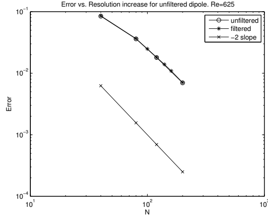
Figure 16: Evolution of error for the filtered and unfiltered simulations.
