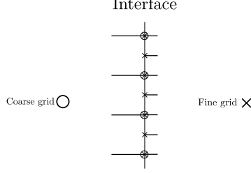
Figure 6: Unknown sites in the fine grid.
