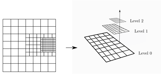
Figure 2: A schematic view the multi-grid approach.
