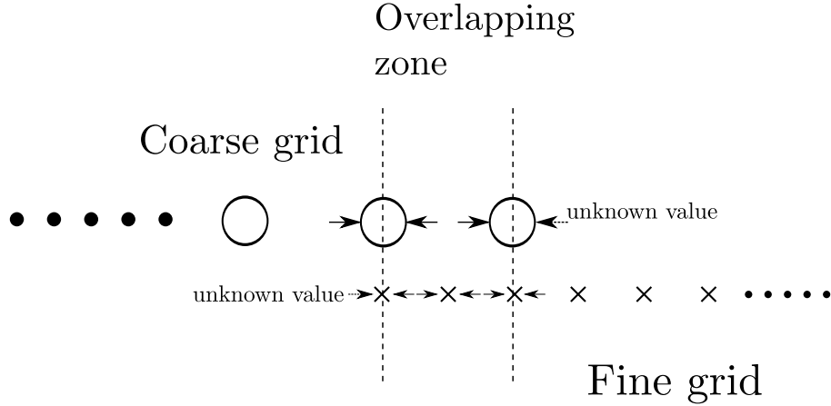
Figure 5: Overlapping zone between coarse and fine grids
