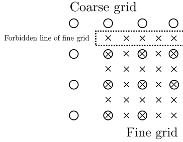
Figure 9: Forbidden case to avoid complicated interpolations.
