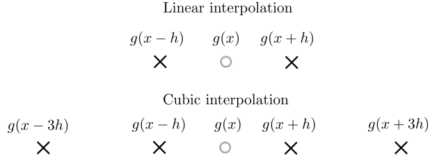
Figure 7: Possible interpolation schemes. Order one (top) and order three (bottom).
