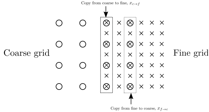
Figure 4: Complete sketch of the places where the copies are performed.
