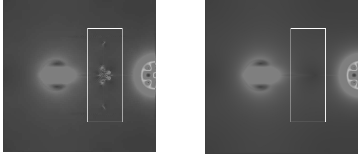
Figure 17: Problems at Re = 5000 for non-filtered simulation on the left. On the right the filtered version, which shows no perturbation.
