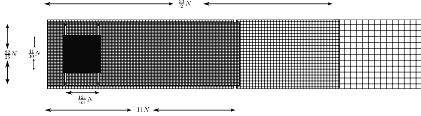
Figure 14: Proposed refinement for the 2D flow past a cylinder.
