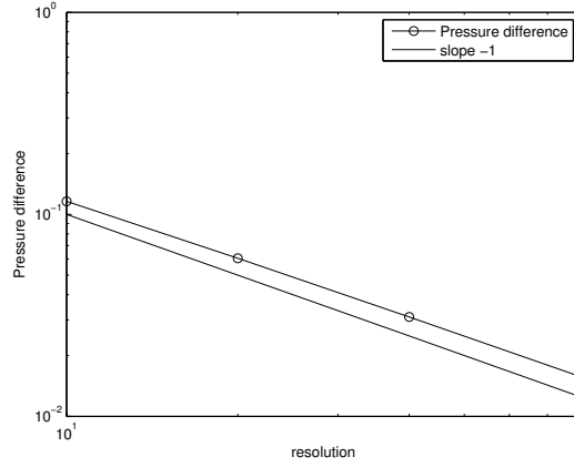
Figure 12: The pressure jump magnitude versus the resolution of the coarse grid.
