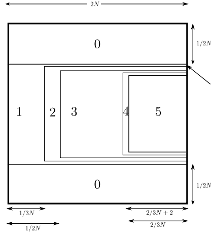
Figure 18: Six level grid refinement to achieve a good enstrophy value.
