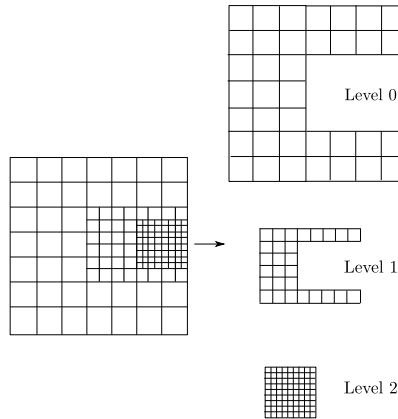
Figure 3: A sketch of the multi-domain approach.
