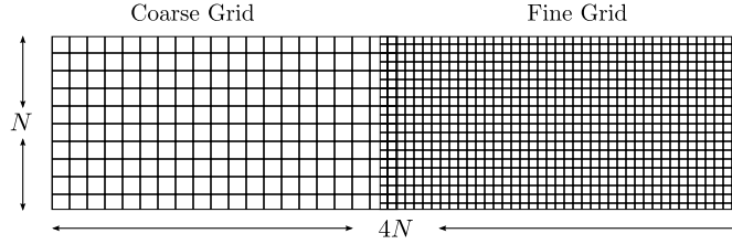
Figure 10: Setup for the channel flow
