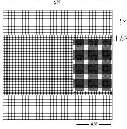
Figure 15: Refinement for the dipole-wall collision
