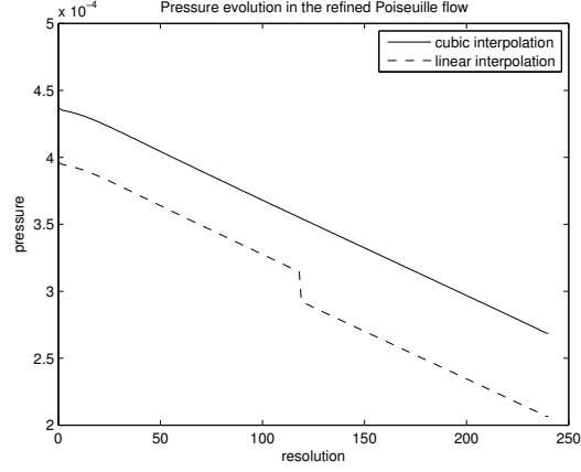
Figure 11: Pressure plot along a horizontal line for the proposed refined Poiseuille flow.
