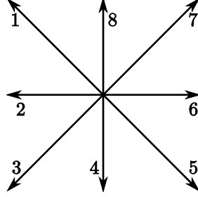
Figure 1: The D2Q9 lattice with the vectors representing the microscopic velocity set \xi_i . A rest velocity \xi_0 = (0, 0) is added to this set.
