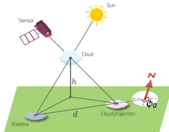
Figure 4. An illustration of cloud and cloud shadow geometry.
