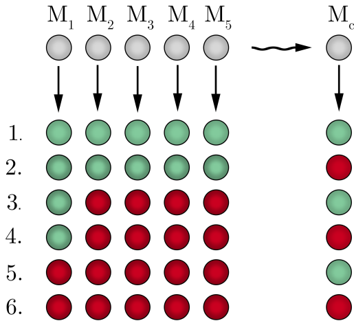
Figure 1: Five dual solutions \mathcal{M}_1, \dots, \mathcal{M}_5 , and their common mathematical core, \mathcal{M}_c . ‘Naïvely interpreted’, such solutions may be understood as representing certain worlds (to which they are ‘isomorphic’—cf. footnote 8). If one such world is green, this indicates that this world is regarded as being a legitimate candidate for being the actual world. If the world is red, on the other hand, this indicates that this world is not regarded as being a legitimate candidate for being the actual world. Options (1)-(6) categorise different verdicts on which of these worlds are regarded as being candidates for being the actual world in this sense.
