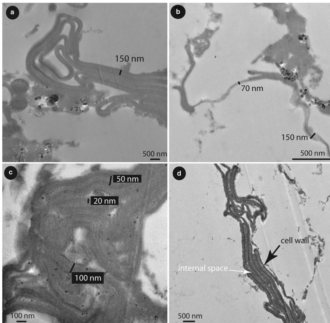
Fig. 15 TEM sections in fossil OM showing a algal cell walls patch of contorted layers in the Urbino level, b bacterial cell walls: thin contorted layers in the Urbino level, c thylakoid membranes contorted pair
