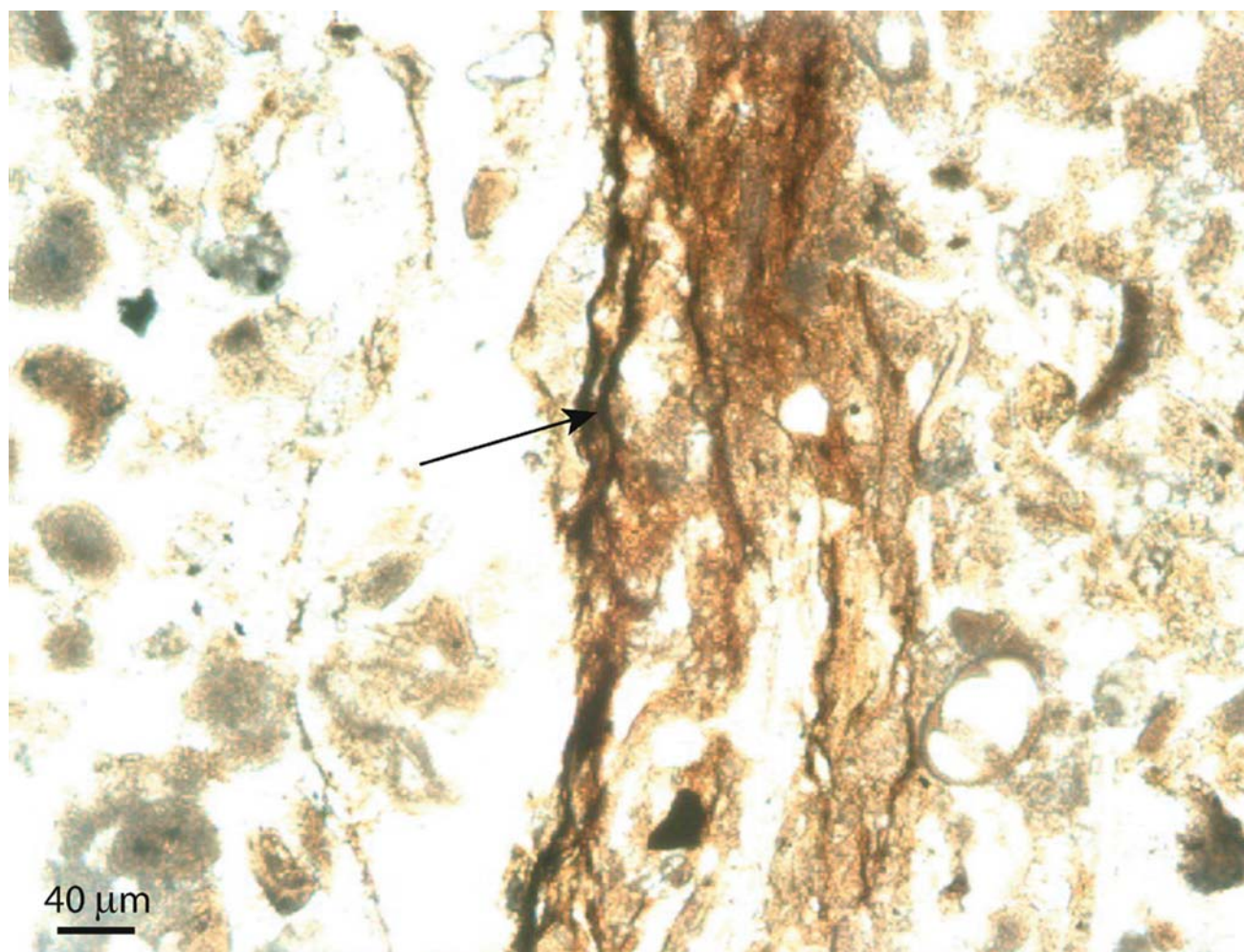
Fig. 6 Petrographic thin section perpendicular to laminations in the recent microbial mat showing organic brown parallel laminae ( black arrow ), organisms and organic clasts
