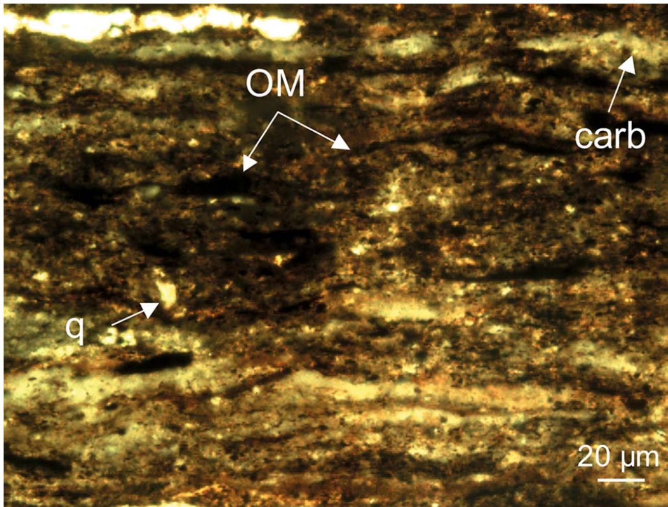
Fig. 5 Petrographic thin section perpendicular to stratification in the Urbino level showing organic-rich laminites with detrital lenses and carbonate grains. Legend: organic matter (OM), quartz (q) and carbonate (carb)
