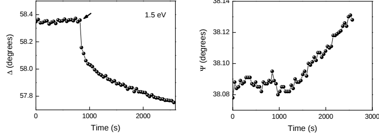
Figure 6.6: The effect of the exposure to the air on the optical properties of \text{MgB}_2 . - The time dependence of ellipsometric parameters \Delta and \Psi at 1.5 eV is shown (sample S1, geometry (caa), angle of incidence 70^\circ ). Initially the sample was kept in a flow of dry nitrogen, which was switched off at the moment designated by the arrow.
