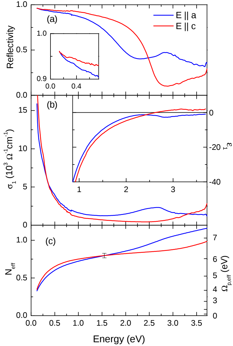
Figure 6.7: Optical anisotropic spectra of \text{MgB}_2 at 300 K derived from the ellipsometry and reflectivity measurements on the sample S1. - (a) The near-normal incidence reflectivity, (b) the optical conductivity and the dielectric function, (c) the effective number of carriers and the effective plasma frequency. The a -axis and the c -axis spectra are shown by the blue and red lines, respectively.
