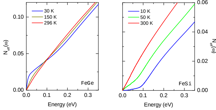
Figure 3.9: The integrated spectral weight for a number of representative temperatures. - For comparison we plot N_{\text{eff}}(\omega) of FeGe (left panel) and N_{\text{eff}}(\omega) of FeSi (right panel) from Ref. [63].
