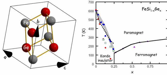
Figure 3.1: B20-type crystal structure of FeGe and the phase diagram of \text{FeSi}_{1-x}\text{Ge}_x . - Left panel: There are four Fe and four Ge ions in a unit cell of FeGe arranged in such way that every atom has seven nearest neighbours of the opposite kind. Gray and red spheres indicate the Fe and Ge atoms, respectively. Right panel: Temperature versus concentration phase diagram of \text{FeSi}_{1-x}\text{Ge}_x from Ref. [2]. A first-order transition from the Kondo insulator phase to a ferromagnetic phase occurs at x \approx 0.25 . For x = 1 the phase diagram corresponds to FeGe.
