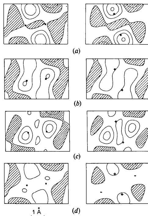
Fig. 3. Residual electron density within the cage. The sections are perpendicular to the crystallographic twofold axis and calculated from the F_c model ( M )-TOT-( R )-EMSO/( S )-EMSO (2: x_R : x_S ). Contour interval 1 \text{ e } \text{\AA}^{-3} , starting at zero contour. Shaded areas: negative density. The equation of the planes passing through the axially disordered S atoms can be expressed as 13.538x - 6.769y = D in direct space. The D value is 4.061 \text{ \AA} for the ( R ) enantiomer (S atoms at ■; left column) and 4.197 \text{ \AA} for the ( S ) enantiomer (S atoms at +; right column). The guest occupancy factor is x_R + x_S = 0.96 . The enantiomeric excess (%) of the ( R ) configuration is calculated as (x_R - x_S) \cdot 100 / (x_R + x_S) : (a) 100%; (b) 83%; (c) 72%; (d) final residual density after refinement of the F_c model with e.e. = 83%. The S-atom positions labelled with + are those originally calculated with the PCK-6 program (Williams, 1972). The final refinement shifts these positions by 0.25 \text{ \AA} away from the twofold axis towards the region of the highest electron density shown in Fig. 3(a).
