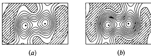
Fig. 2. Sections through three-dimensional \Delta F syntheses in the plane containing the axially disordered S atoms (■) of ( R )-ethyl methyl sulfoxide. Contours at intervals of 1 \text{ e } \text{\AA}^{-3} ; negative contours dashed. (a) Calculated on the basis of the refined model ( M )-TOT-( R )-EMSO (2:1) with F_c from which the contribution of the guest had been omitted; (b) F_c calculated from the host structure refined to convergence limit without inclusion of the guest.
