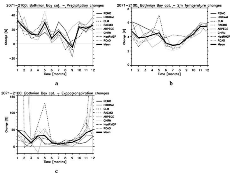
Fig. 5 Change in a precipitation, b 2 m temperature and c evapotranspiration from RCM-H/A2 scenario simulations for the Bothnian Bay Basin. The pronounced percent increases in c for some models reflects the relatively small evapotranspiration values generated for the control climate
