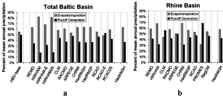
Fig. 3 RCM partitioning of precipitation into evapotranspiration and runoff generation over a the total Baltic Basin and b the Rhine Basin. All used HadAM3H boundary conditions with the exception of two that used ECHAM4/OPYC3 (marked with “E”). HBV-Baltic results using observations are also shown in a (HBV-base)
