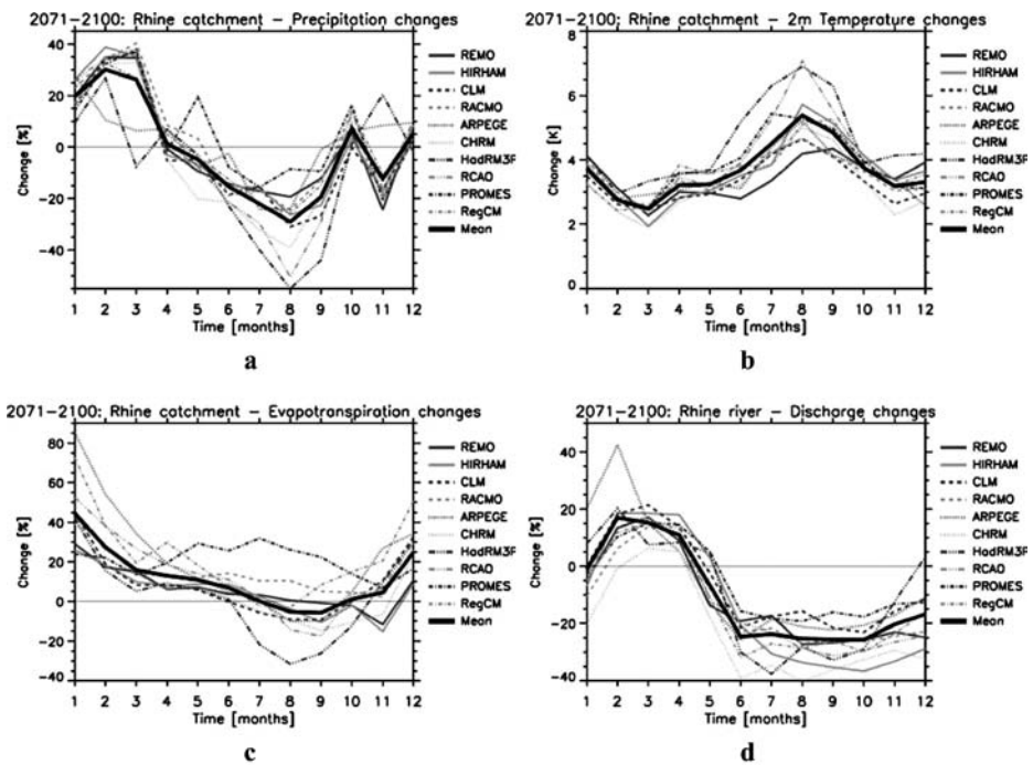
Fig. 12 Change in a precipitation, b 2 m temperature, c evapotranspiration and d HD Model routed river discharge from RCM-H/A2 scenario simulations for the Rhine Basin
