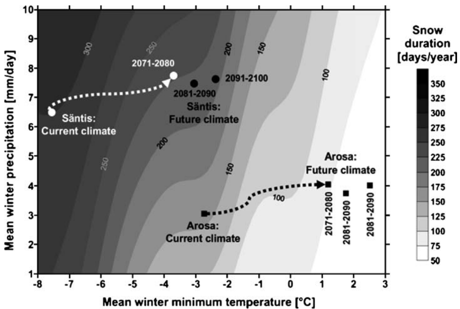
Fig. 16 2-D contour surfaces of snow cover duration as a function of winter (DJF) minimum temperature and precipitation, based on climatological data from 20 sites in Switzerland. The numbered isolines refer to the length of the snow season in days. Superimposed on the contour surface is temperature/precipitation/snow-duration data for Arosa (1,865 m.a.s.l.) and Sântis (2,500 m.a.s.l.) for both current climate conditions and projections of the last three decades of the twenty-first century. Arrows indicate change from current to future climate conditions
