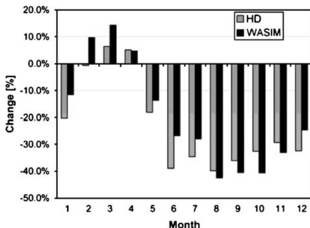
Fig. 14 Comparison of WASIM and HD Model generated Rhine river discharge changes at Cologne using the CHRM-H/A2 scenario
