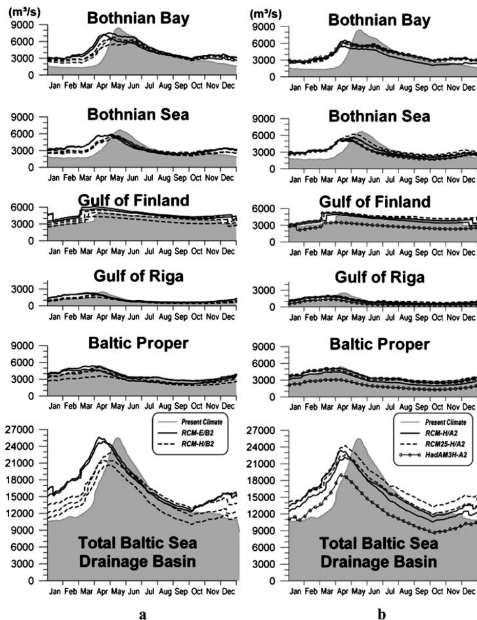
Fig. 7 Mean daily river discharge from HBV-Baltic using the delta approach for a RCM-B2 scenarios at ~50 km resolution driven by HadAM3H and ECHAM4/OPYC3, and b RCM-A2 scenarios driven by HadAM3H at resolutions of ~25 and ~50 km, and HadAM3H at ~150 km. Shown in gray shading is the present climate
