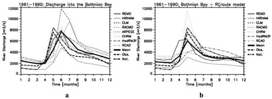
Fig. 4 Routed river discharge from RCM control simulations for the Bothnian Bay Basin from a HD Model and b RCroute
