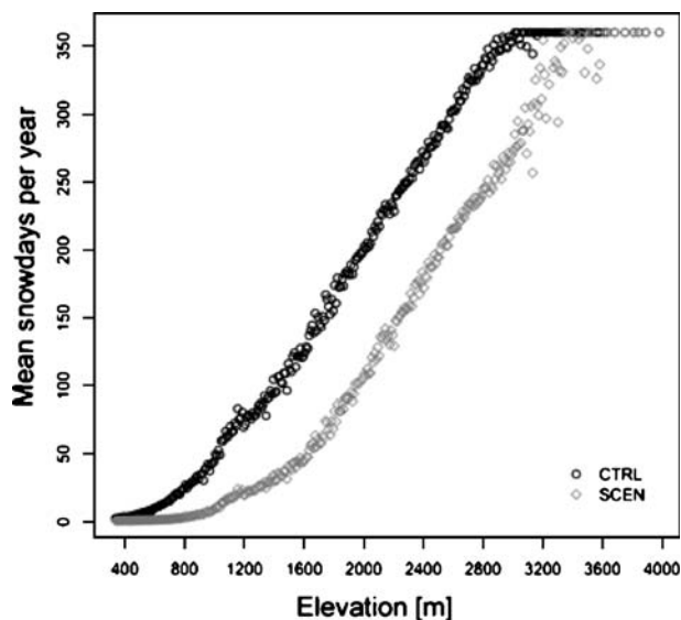
Fig. 15 Snow duration versus elevation from WASIM-CTRL and WASIM-H/A2 simulations for the combined Alpine area of Aare, Limmat, Reuss and Rhine subbasins
