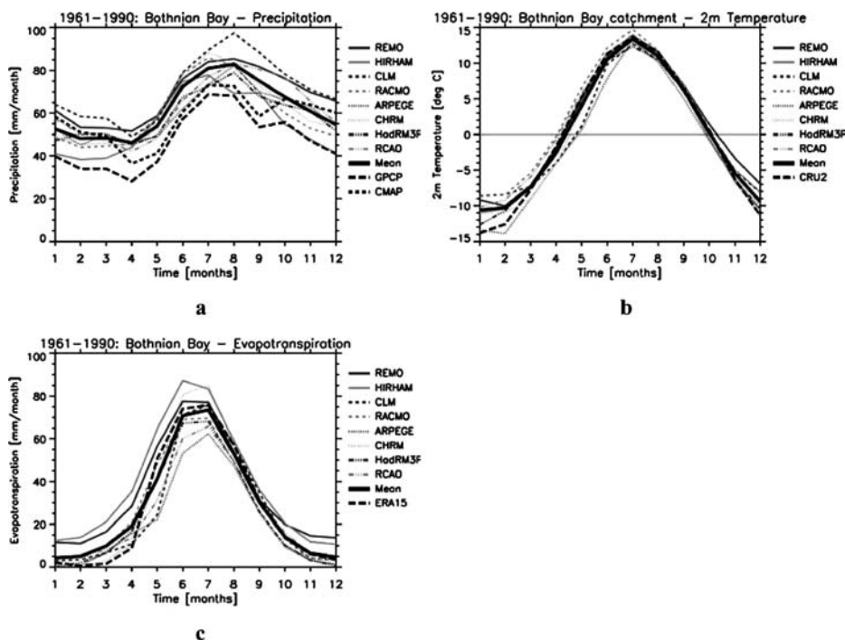
Fig. 2 a Precipitation, b 2 m temperature and c evapotranspiration from RCM control simulations for the Bothnian Bay Basin
