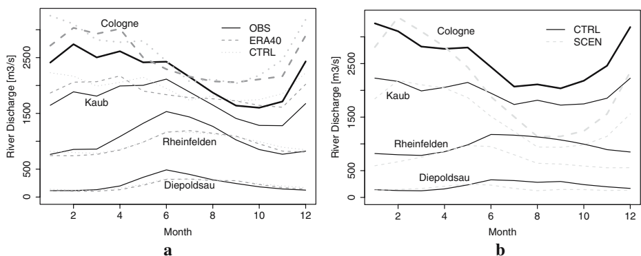
Fig. 13 Mean monthly river discharge at four locations along the Rhine River for a the WASIM-CTRL and WASIM-ERA40 simulations, and b the WASIM-H/A2 simulation. Cologne is shown with bolder lines to emphasize that it is the most downstream location
