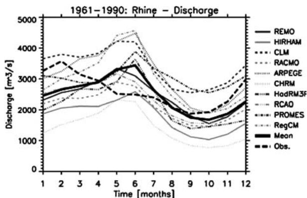
Fig. 11 HD Model routed river discharge from RCM control simulations for the Rhine Basin
