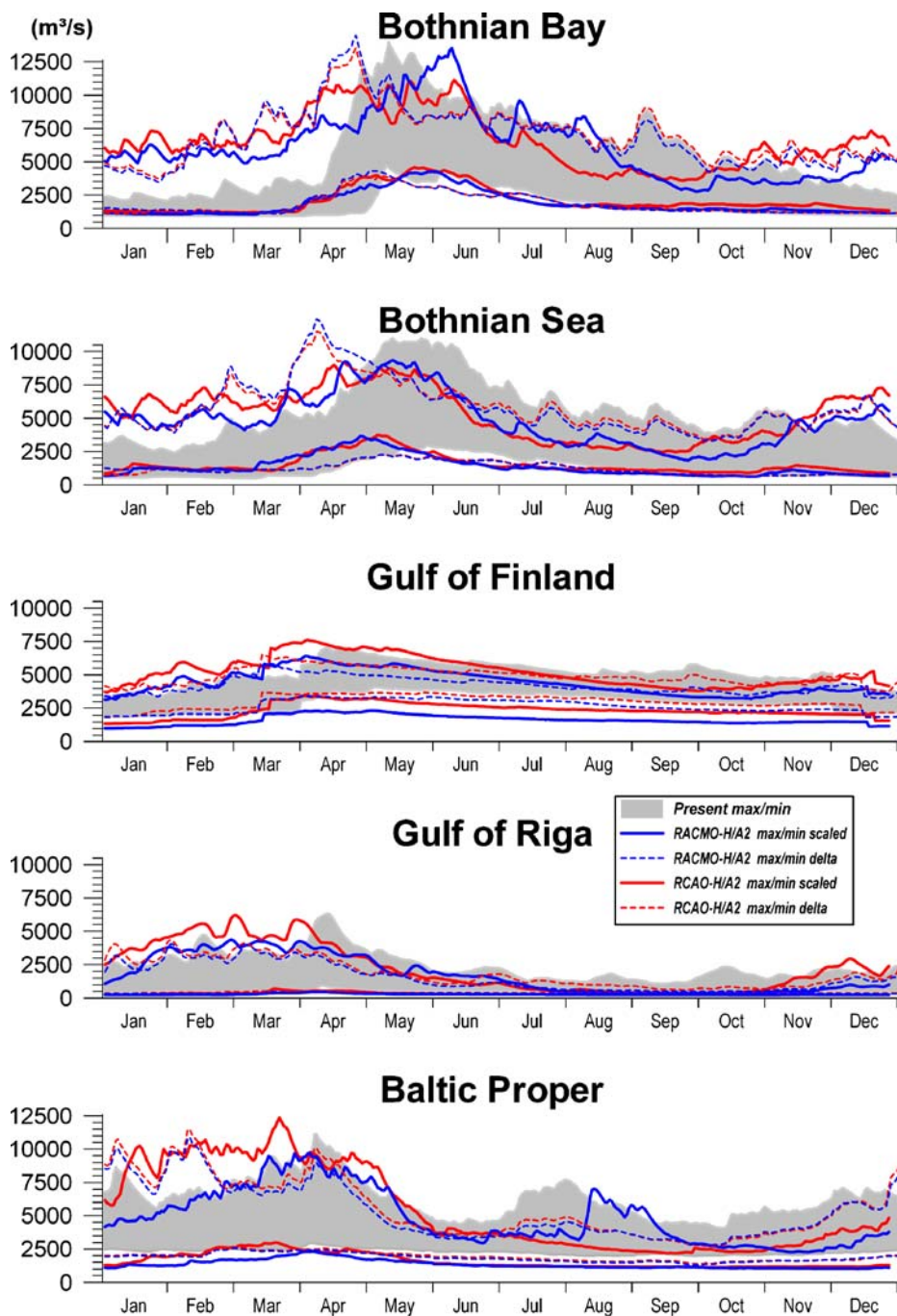
Fig. 9 Model period maximum and minimum daily river discharge from HBV-Baltic using both the precipitation scaling approach and the delta approach for two RCMs (RACMO and RCAO) driven by the HadAM3H-A2 scenario. Shown in gray shading are corresponding maximum and minimum values for the present climate
