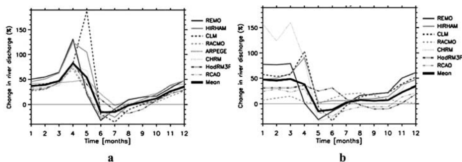
Fig. 10 Percent change in routed river discharge from RCM-A2 scenario simulations for the Bothnian Bay Basin from a HD Model and b RCroute
