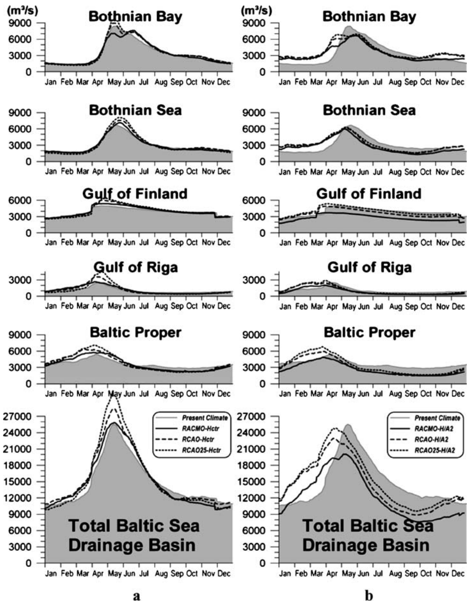
Fig. 8 Mean daily river discharge from HBV-Baltic using the precipitation scaling approach for three RCMs driven by HadAM3H-A2 for a control simulation, and b scenario simulation. Shown in gray shading is the present climate
