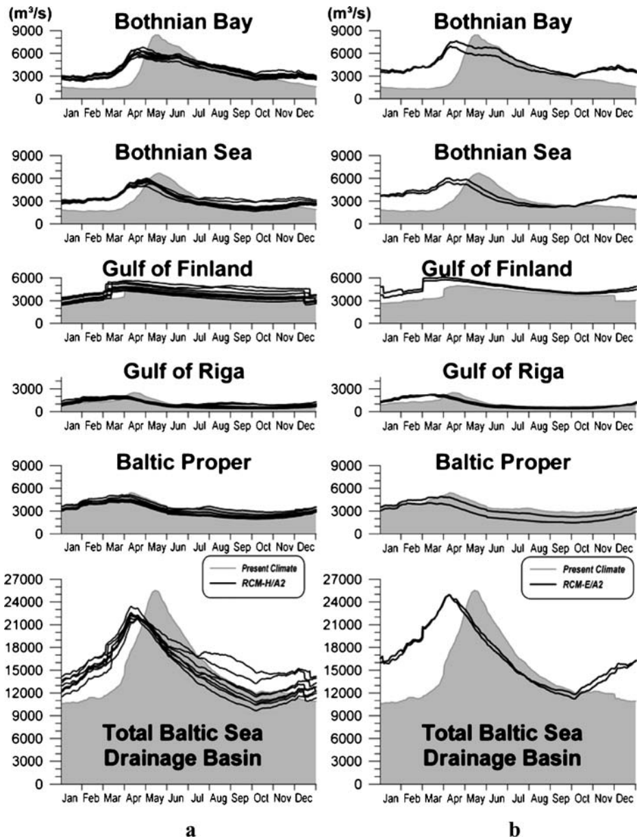
Fig. 6 Mean daily river discharge from HBV-Baltic using the delta approach for RCM-A2 scenarios at ~50 km resolution, driven by a HadAM3H and b ECHAM4/OPYC3. Shown in gray shading is the present climate
