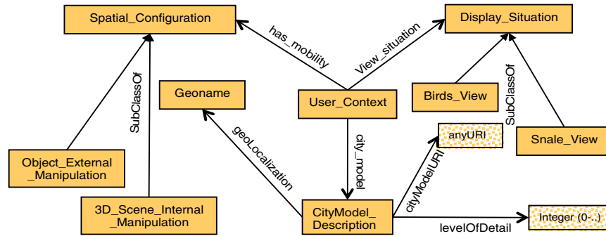
Figure 6. Specifications and representation of the User_Context concept.
