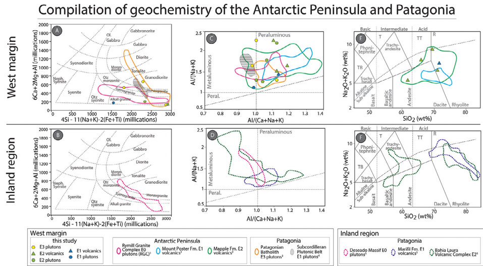
Fig. 3. Geochemical compilation showing the relevant classification diagrams for the igneous rocks of the Antarctic Peninsula and Patagonia. This figure has been divided between Inland Region and West Margin units throughout the Late Triassic – Jurassic. Source of the data: 1 – [6,7], 2 – [2], 3 – [4], 4 – [3], 5 – [5].
