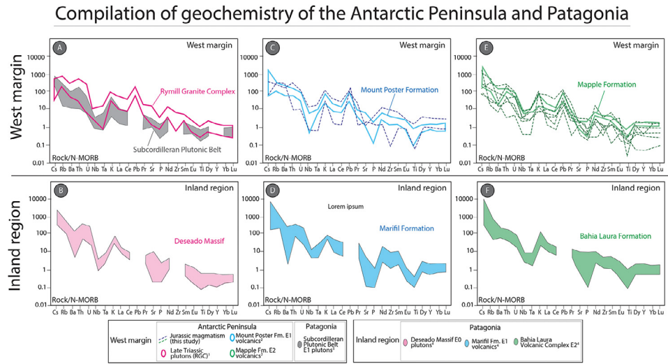
Fig. 4. Geochemical compilation showing trace element abundances normalized to N-MORB (values from [26]) for the igneous rocks of the Antarctic Peninsula and Patagonia. This figure has been divided between Inland Region and West Margin units throughout the Late Triassic – Jurassic. Source of the data: 1 – [1,6,7], 2 – [2], 3 – [3], 4 – [5].
