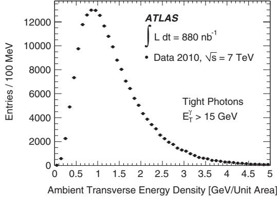
FIG. 1. The measured ambient-transverse-energy densities, using the jet-area method, for events with at least one tight photon. The ambient-transverse-energy contains contributions from both the underlying event and pile-up. The broad distribution reflects the large event-to-event fluctuations.
