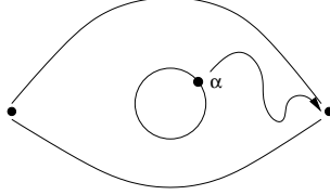
FIGURE 8. A simple path from Duflou-Kontsevich star product to standard product
