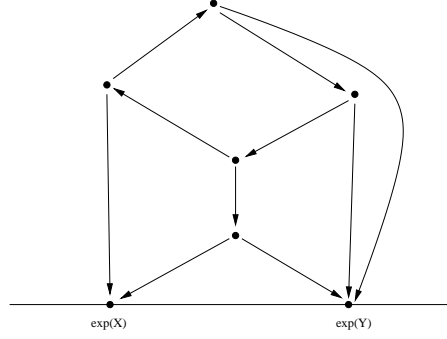
FIGURE 3. Wheel type graph with symbol \Gamma(x, y) = \text{tr}(y^2[x, y]x) .
