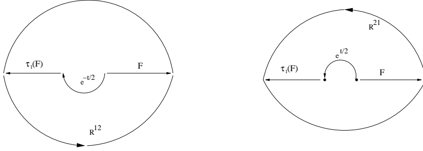
FIGURE 9. The R matrix
