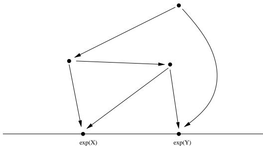
FIGURE 2. Lie type graph with symbol \Gamma(x, y) = [[x, [x, y]], y] .
