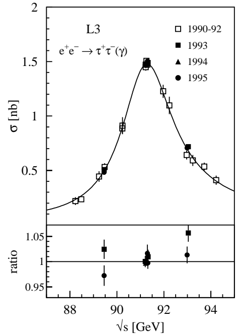
Fig. 26. Same as Fig. 24 for e^+e^- \rightarrow \tau^+\tau^-(\gamma)
