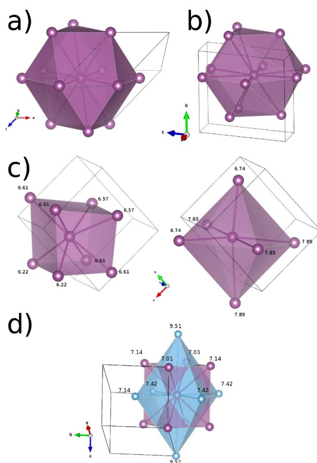
Figure 2. Anion–anion coordination for (a) monoclinic rt - \text{Na}_2\text{B}_{12}\text{H}_{12} with cubic close packing ( ccp ) of anions. The first coordination sphere contains 12 nearest neighbors at the distance 7.01–7.42 Å forming
