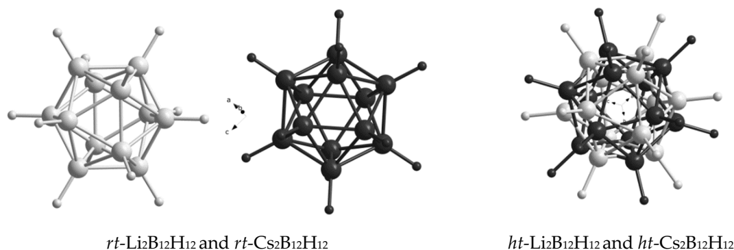
Figure 3. Two orientations, dark and light gray, of the closo -anion in the rt ordered (s.g. Pa -3) and in the ht disordered \text{Li}_2\text{B}_{12}\text{H}_{12} (s.g. Fm -3) viewed along the C_3 rotation axis of the closo -anion. The rt\text{-Cs}_2\text{B}_{12}\text{H}_{12} (s.g. Fm -3) contains one anion in the orientation identical to the light gray anion in rt\text{-Li}_2\text{B}_{12}\text{H}_{12} , while the ht\text{-Cs}_2\text{B}_{12}\text{H}_{12} (s.g. Fm -3 m ) has an identical orientation disorder (rotation around C_3 by 45^\circ ) as ht\text{-Li}_2\text{B}_{12}\text{H}_{12} .
