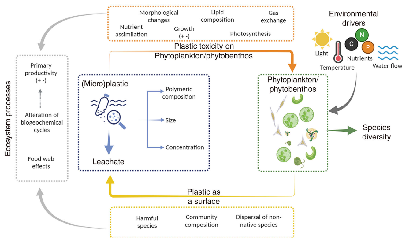
Fig. 4. Representation of the interaction between phytoplankton/phytobenthos, (micro)plastics and environmental factors (e.g. light, nutrients, temperature), and their subsequent effects on wider ecosystem processes. The effects of microplastics depend on their size, concentration, and polymeric composition, and by their leachates. These interactions may have toxic effects on phytoplankton/phytobenthos, that is morphological changes, alterations in nutrient assimilation, shifts in gas exchange, increased production of fatty acids, and impacts on growth and photosynthetic activity. The phytoplankton/phytobenthos–plastic interaction also involves effects linked to plastics serving as a surface for algal colonisation. (Micro) plastics can potentially influence community composition, provide a habitat for harmful species, and act as a vector for non-native species. Together, both toxicity and provision of a substrate for growth by (micro) plastics can impact crucial ecological processes, including primary productivity and nutrient cycling, with possible repercussions throughout the entire aquatic food web. \pm denotes instances where the effects may be positive or negative.
